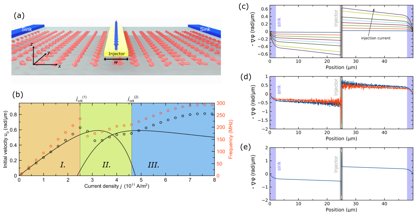
FIG. 1. EMS in the absence of dipolar interaction. (a) Schematic view of the thin film. The spin injector provides spin current with out-of-plane polarization (blue arrows). The spin sinks are shown. The red arrows represent a magnetization snapshot. (b) Initial EMS velocity (black circles) and base frequency (red circles) as functions of the current density. Three regimes of the EMS are marked. Black line shows transmitted spin current \tau (in the same units as EMS velocity) calculated based on the analytical model. (c) Spatial dependence of the EMS velocity in regime I, (d) in regime II at j = 3.1 \cdot 10^{11} A m ^{-2} , (e) in regime III at j = 4.6 \cdot 10^{11} A m ^{-2} .
