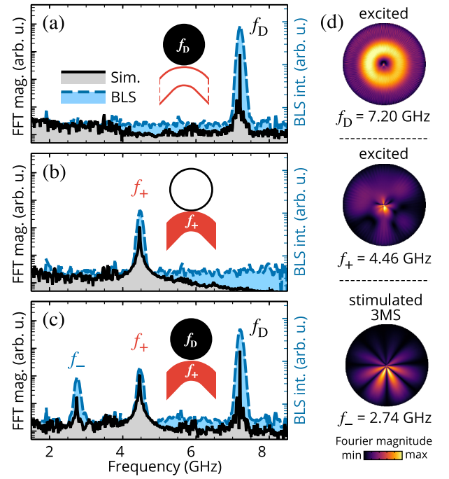
FIG. 2. Spectra of the vortex disk obtained by micromagnetic simulations and \mu\text{BLS} for three cases: (a) only the disk is excited below threshold at frequency f_D , (b) only the waveguide is excited at frequency f_+ and (c) both combined, showing an additional signal at f_- . (d) mode profiles obtained from the simulation in (c).
