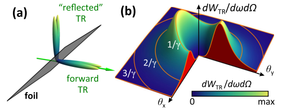
FIG. 10 Color online. Angular distribution of TR power for relativistic electrons incident at 45^\circ on foil: (a) “reflected” and forward TR cones; (b) far-field distribution of one cone, showing break in azimuthal symmetry.
