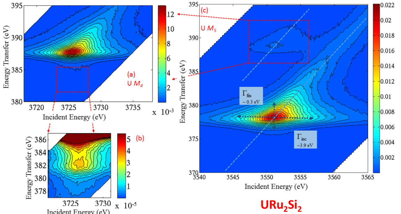
FIG. 5. Full data from RXES experiments at M_4 (left) and M_5 (right) from \text{URu}_2\text{Si}_2 .
