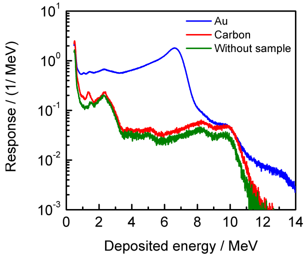
FIG. 20. Distribution of the energy deposited in the BaF 2 detector installed at n_TOF. The results of measurements with a Au and carbon sample are compared with the one without sample. The data are from Ref. [99].
