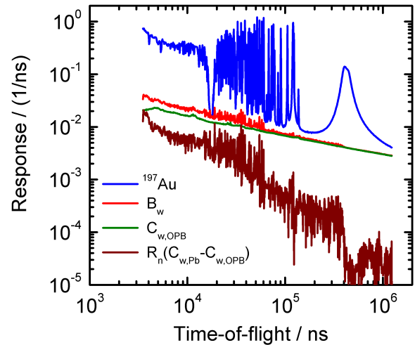
FIG. 22. The response of a C_6D_6 detector system as a function of TOF for a 1.0 mm {}^{197}\text{Au} sample [198] obtained at GELINA is compared with the contribution of the different background components.
