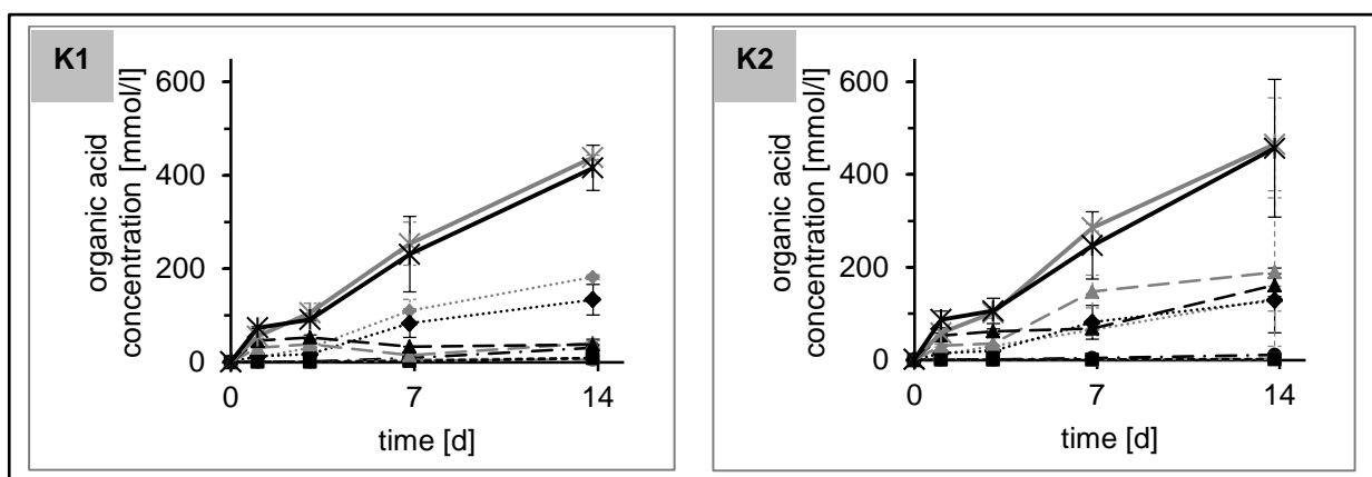
Fig.6: Exemplary depiction of organic acid production in Kombucha-cultures during leaching of FP. Left: stationary, right: shaken cultivation. X...Overall COOH production, \Delta ...acetic acid, \diamond ...gluconic acid, \circ ...citric acid, \square ...tartaric acid; grey: control with microorganisms, black: sample with microorganisms and FP.
