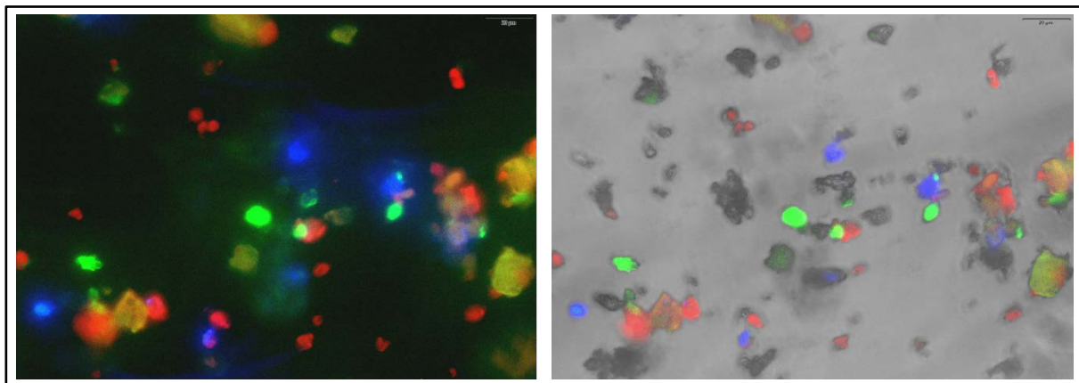
Fig. 2: Fluorescence microscopic analysis of the used FP. Left: Overlay of different fluorescent microscopic pictures, right: additional overlay of light microscopic picture. Particles belong to blue, green and red triband dyes, as well as white halophosphates and supporting substances.
