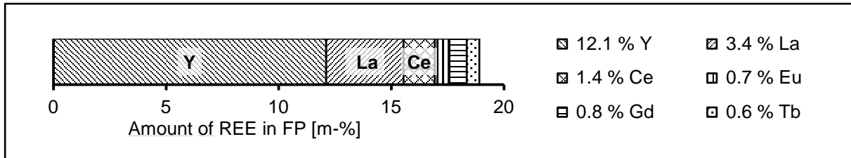
Fig.1: Elemental composition of the used FP measured by XRF in weight-%.
