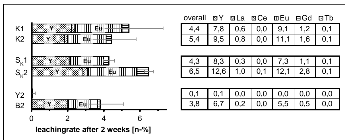
Fig. 5: Comparison of relative molar leaching rate of REE minus the leaching effect of the medium after 2 weeks in mole-%. K: cultivation of whole Kombucha on Kombucha-media, S_K : cultivation supernatant of a two weeks lasting cultivation, Y: yeast isolate of Kombucha on YPD media, B: bacteria isolate on DMSZ media 105, 1: stationary, 2: shaken inkubation.
