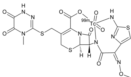
Figure 4. Proposed structure of 99m Tc-cefttriaxone 72
