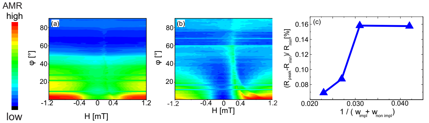
FIG. 6. Measurement of the AMR at different field angles \varphi for (a) a permalloy film and (b) a stripe sample with w=16 [16 \mu\text{m} (implanted | non-implanted) stripes]. (c) Dependence of the height of the extra peak at the interface on the sum of implanted and non-implanted stripe width ( w_{\text{imp}}|w_{\text{nonimp}} ).
