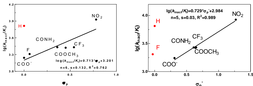
Figure 6. Relationship between the electronic properties ( \sigma_p and \sigma_p^- ) of the substituents in position 6 of the pyridin-3-yl moiety and the inactivation constants of the inhibitors 8a-g
