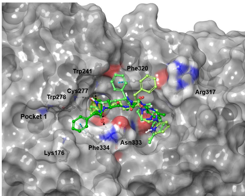
Figure S6: Molecular modelling of the interaction of hTGase 2 with 6a
