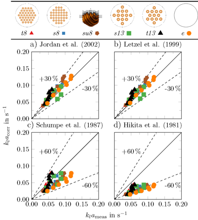
Figure 13: Parity plots comparing volumetric gas-liquid mass transfer coefficients from this study with predictions of available correlations from a) Jordan et al. (2002) b) Letzel et al. (1999) c) Schumpe et al. (1987) and d) Hikita et al. (1981).
