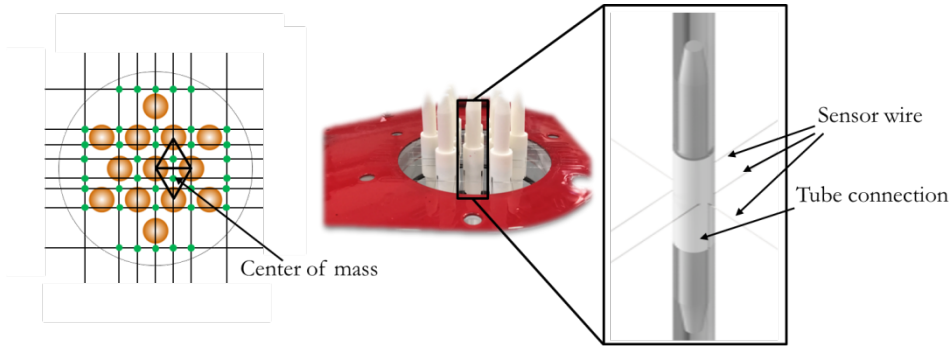
Figure 2: WMS electrode configurations for the different tube arrangements (top) and photography of the sensor for the triangular 13 ( t13 ) configuration with zoomed view of an inlay that is part of the tube mockup and serves as a support for wire electrodes and a spacer for the tubes (bottom).
