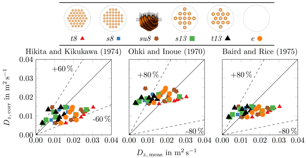
Figure 12: Parity plots comparing axial dispersion coefficients from this study with predictions of available correlations for superficial gas velocities up to 0.08 \text{ m s}^{-1} .
