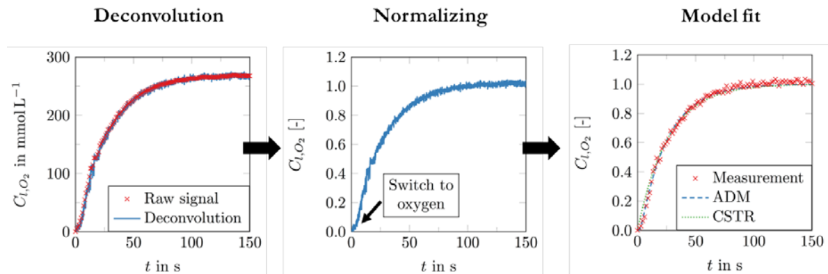
Figure 4: Illustration of the oxygen probe data post-processing and model fitting steps.
