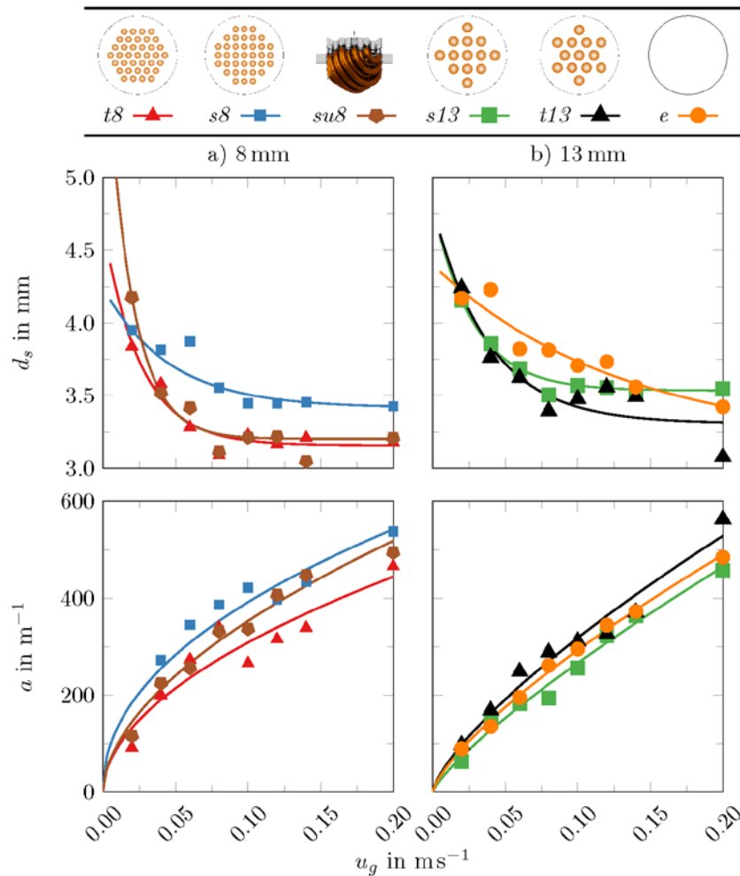
Figure 11: Sauter mean diameter (top row) and interfacial area (bottom row) as a function of the superficial gas velocity for the various internals as well as for the empty bubble column.
