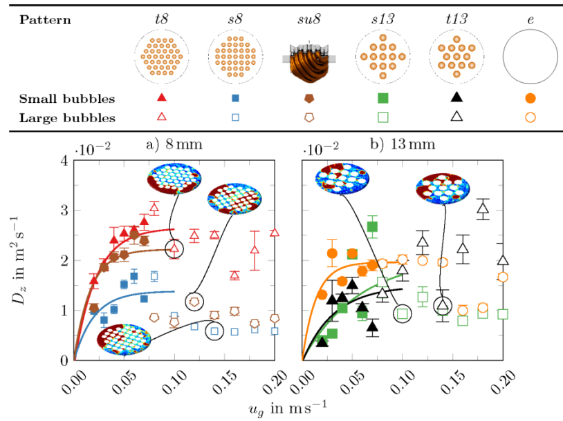
Figure 6: Effect of the superficial gas velocity on the liquid axial dispersion coefficient for the various tube bundles (tomographic cross-sectional images show large bubbles, indicated by dark red color, passing the measurement plane). Note that the y-axis has to be multiplied by 10^{-2} .
