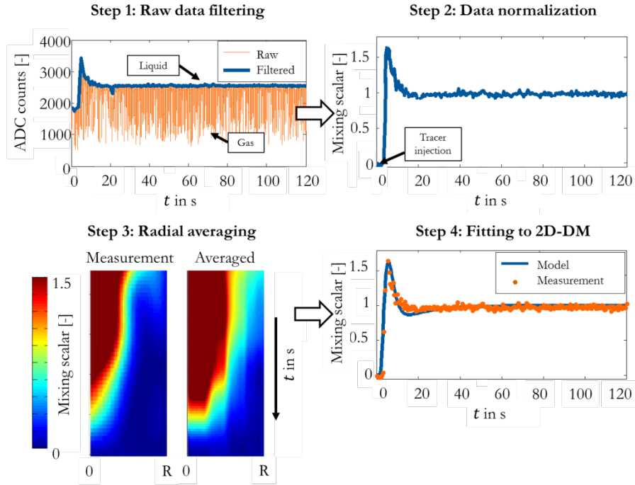
Figure 3: WMS data post-processing procedure and dispersion parameter extraction (data in step 1 and 2 shown for one virtual crossing point only, data in step 4 shown for one radius only).
