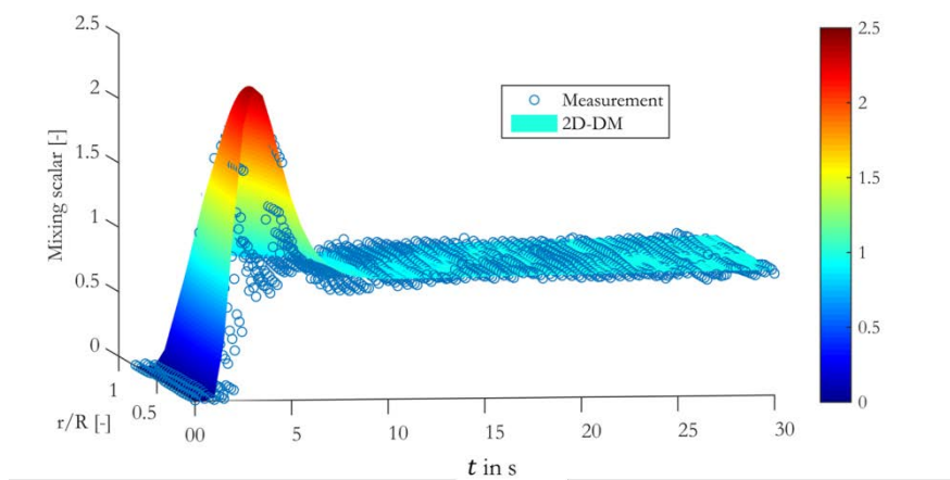
Figure 5: Fit of the 2D dispersion model solution to experimental data for the square 8 configuration with U-tube bottom end design ( su\delta ) at a superficial gas velocity of 0.04\text{ m s}^{-1} .
