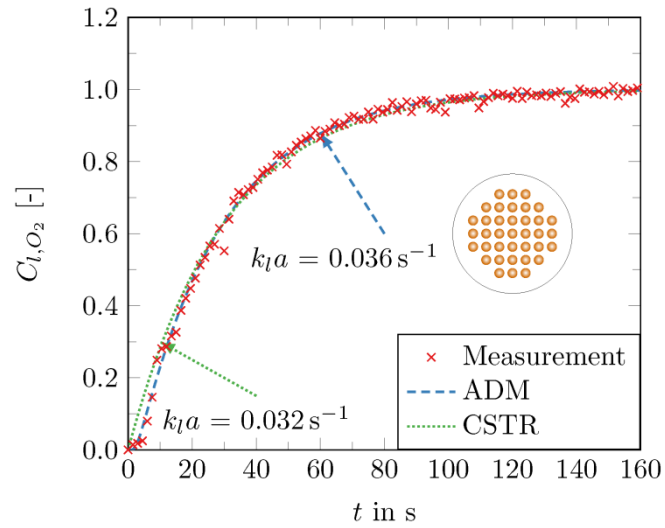
Figure 8: Temporal concentration profile obtained with the CSTR model and the ADM for the square 8 ( s\theta ) configuration at a superficial gas velocity of 0.02\text{ m s}^{-1} .
