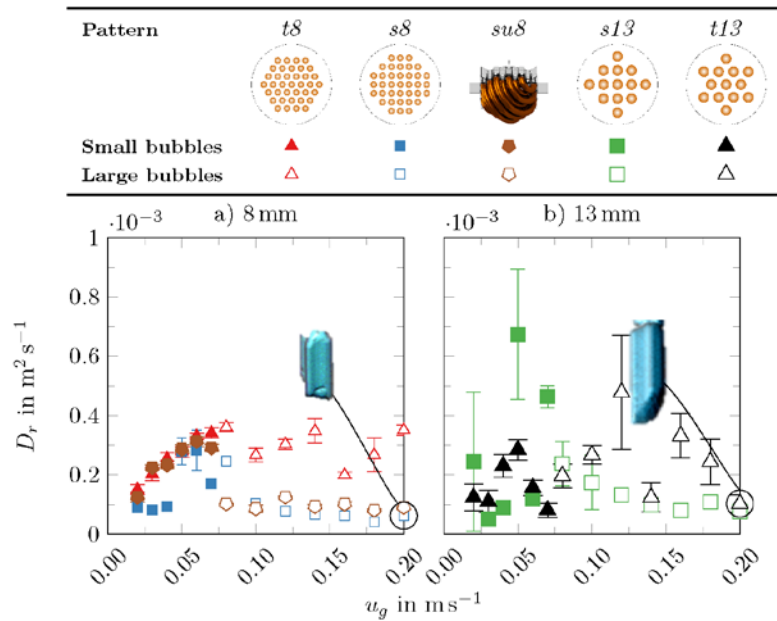
Figure 7: Radial liquid dispersion coefficient as a function of the superficial gas velocity for the various tube bundles (3D inserts show the formation of elongated bubbles in the sub-channels obtained from ultrafast X-ray tomography). Note that the y-axis has to be multiplied by 10^{-3} .
