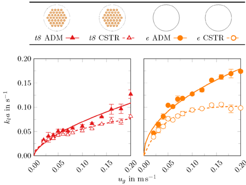
Figure 10: Volumetric mass transfer coefficient obtained with the ADM and the CSTR model for the packed and empty bubble column.
