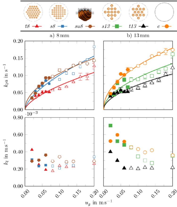
Figure 9: Volumetric mass transfer coefficient (top row) and liquid-side mass transfer coefficient (bottom row) as a function of the superficial gas velocity for a) 8 mm tubes as well as the U-tube bottom end structure and b) 13 mm tubes as well as the empty counterpart.
