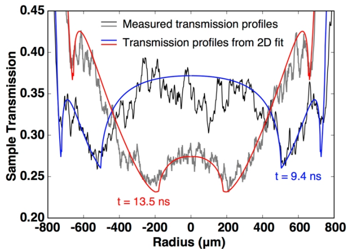
FIG. 4: Comparison of the measured and inferred sample transmission profiles that correspond to the inferred mass density profiles shown in Fig. 3.
