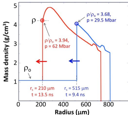
FIG. 3: Inferred radial mass density profiles at two different times as the shock moves inwards. Inside the shock is the pristine polystyrene sample at solid density of \rho_0 = 1.085 \text{ g/cm}^3 .
