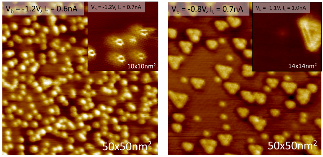
Figure 3. STM studies of MoTe 2 surfaces with Mo deposited at room temperature and subsequent annealing. (a) Large scale STM images of MoTe 2 after Mo deposition at room temperature. The inset shows the structure of individual Mo-induced point defects (likely Mo-interstitials). (b) Large scale STM images of MoTe 2 after annealing at 250°C. Annealing at such temperature converts the point defect into MTB-loops clearly resolved in the inset.
