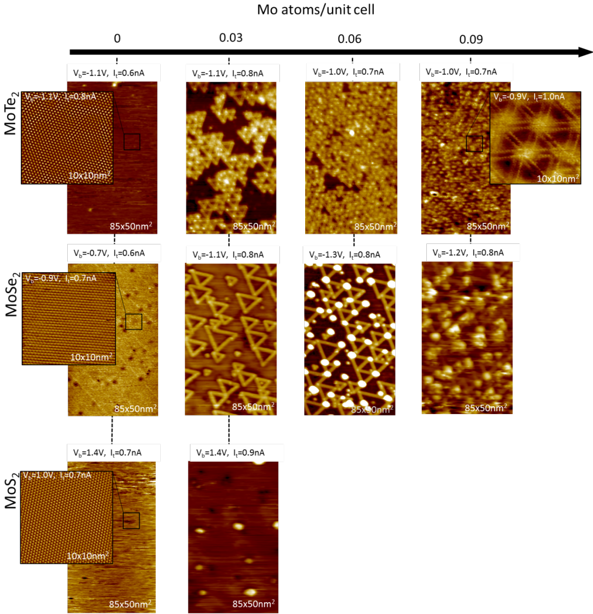
Figure 2. STM images for sequential deposition of Mo at 350°C on the three different Mo-dichalcogenides substrates. The axis is based on the normalized number of Mo atoms absorbed within the unit cell of MoTe 2 .
