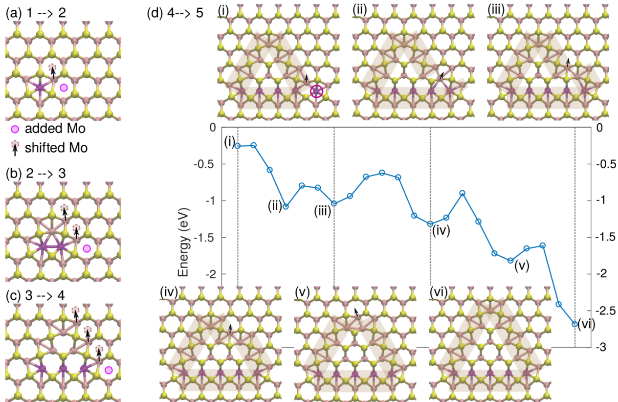
Figure 6. Illustration and energy barriers for the growth of a MTB-loop by addition of an extra excess Mo atom. (a-d) Illustration of the atomic mechanism for the enlargement of the MTB loop (from size N to N+1 ) by addition of excess Mo (magenta atoms). The magenta circle denotes the position of the next added Mo and the black arrow the subsequent shift of the neighboring Mo atom(s) with the final position shown by brown circles. (d) Atomic configurations and the corresponding energy landscape for the transformation from N=4 to N=5 , showing overall decrease in energy. All barriers between local energy minima are within 0.2 - 0.5 eV. Zero energy corresponds to MTB loop of size N=4 and isolated Mo interstitial, indicating that the corner site is more favorable.
