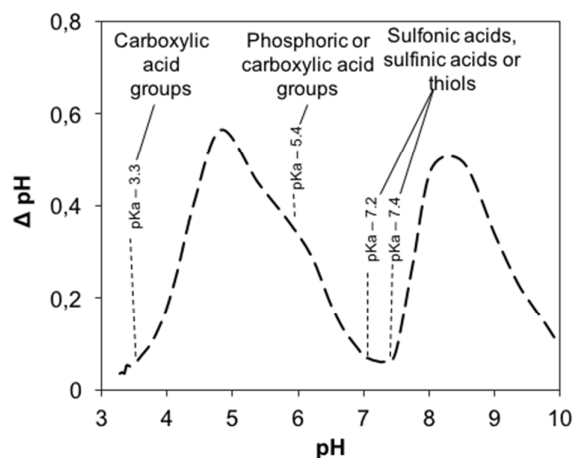
Figure 2. Derivative of acid-base titration data to identify the functional groups present on the surface of BioSe-Nanorods
