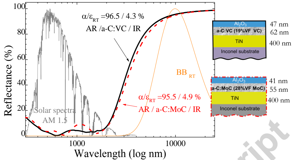
Figure 11: Simulated reflectance spectra of \text{Al}_2\text{O}_3/\text{a-C:VC (19\%VF VC)}/\text{TiN} and \text{Al}_2\text{O}_3/\text{a-C:MoC (28\%VF MoC)}/\text{TiN} of the optimized solar selective coatings. The solar spectrum (AM1.5) and the black body radiation at 25°C (Planck's law) are included.
