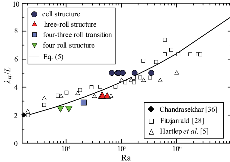
FIG. 11. Horizontal wavelength of the large-scale circulations \lambda_{\text{H}} versus \text{Ra} , where the solid line indicates relation \lambda_{\text{H}}/L = 1.60\text{Ra}^{0.12} - 2 ; symbols of open triangle and open square are from Hartlep et al. [5] and Fitzjarrald [28] obtained in air layers ( \text{Pr} \sim 0.7 ) and a symbol black diamond is the critical wavelength \lambda_{\text{Hc}}/L = 2.016 at \text{Ra}_c = 1708 from Chandrasekhar [36].
