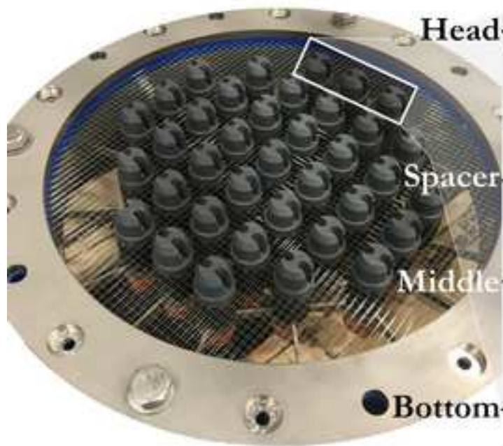
Wire-mesh sensor
