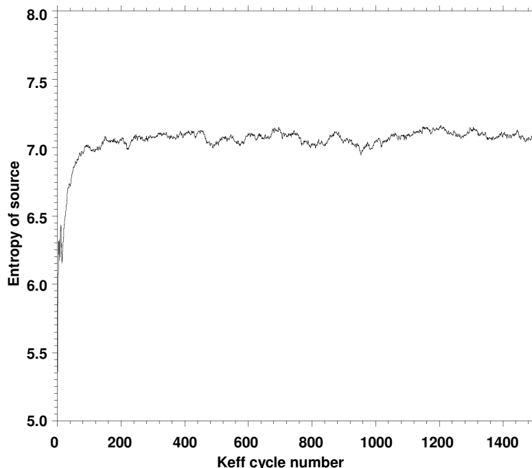
Fig. 6: Convergence of the Shannon entropy of a neutron source term over the cycles (gap width of 0.5 cm, boron concentration of 500ppm and fresh fuel assemblies)
