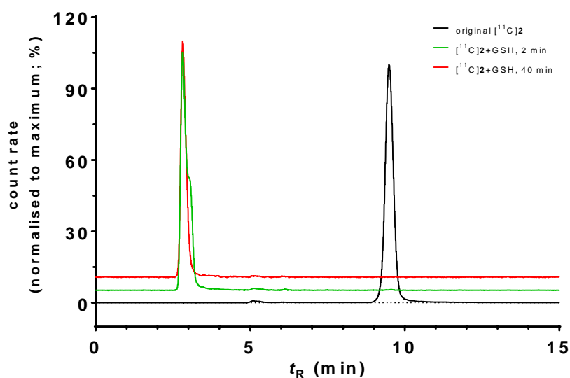
Figure 7: Conjugate formation between azadipeptide nitrile [^{11}\text{C}]\mathbf{2} and glutathione as demonstrated by radio-HPLC. For better visualisation, radio-HPLC chromatograms for 2 and 40 min were shifted 5 and 10%, respectively, at the ordinate.
