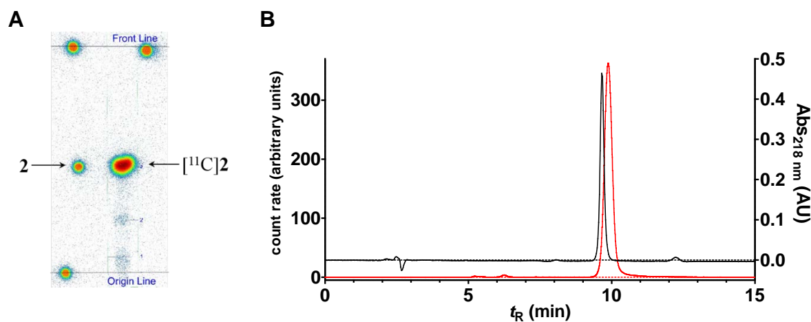
Figure 4: Proof of identity and radiochemical purity of [^{11}\text{C}]\mathbf{2} by analytical radio-chromatography. A) radio-TLC of the final product (right) and the reference compound (left) spotted with radioactivity after UV -visualisation, B) radio-HPLC (red trace) overlaid with the HPLC chromatogram of \mathbf{2} monitored at 218 nm.
