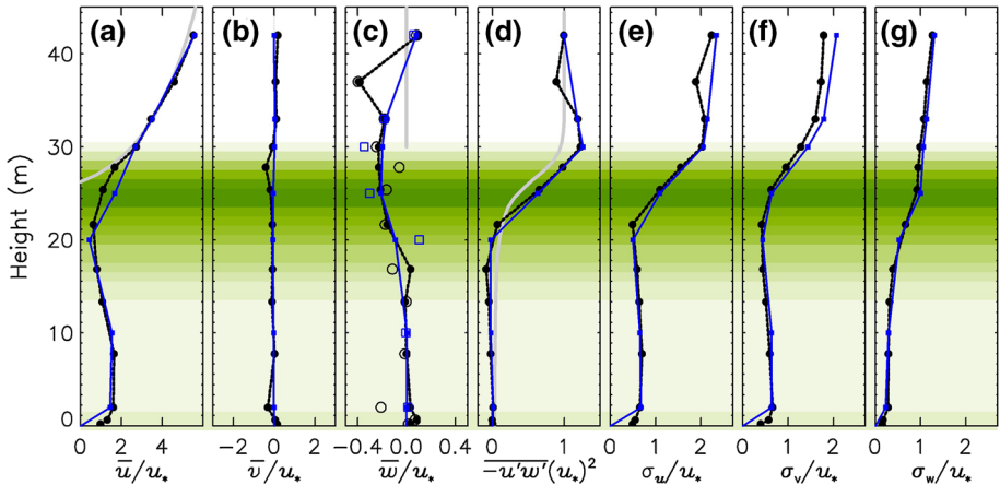
Fig. 5 Comparison of the statistics from the experiments WinCanop ( dashed black line with points ) and TurbEFA ( solid blue line with horizontal marks ). The mean profiles are calculated from near-neutral situations with westerly winds between 3.8 \text{ m s}^{-1} and 4.2 \text{ m s}^{-1} . The plots show mean values normalized with the friction velocity u_* : a–c velocity components (note the different scales of the x -axes for the vertical velocity), d Reynolds stress, e–g standard deviations of the velocity components. For comparison, theoretical functions of the canopy structure are included: a the logarithmic wind profile using a displacement height of 24 m and a roughness length of 2.2 m and d the function \overline{u'w'} = \exp(-0.5PAC) according to Yi (2008), where PAC is the cumulative single-sided plant area density
