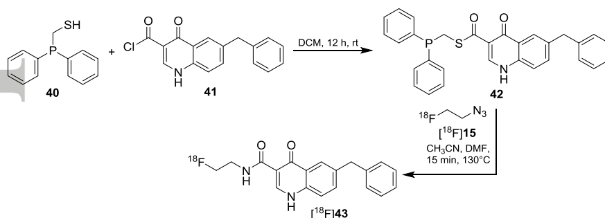
Scheme 15. Preparation of radiotracer [ 18 F] 43 for imaging of GABA A receptor.
