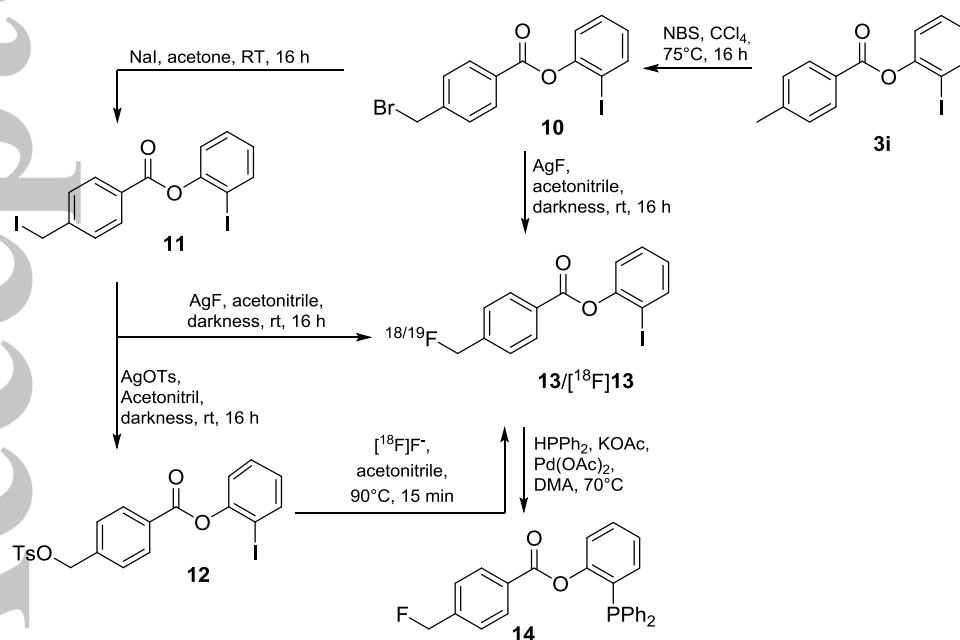
Scheme 10. Preparation of precursors 10 , 11 , and 12 , and the fluoromethyl-containing phosphanes 13 , [ 18 F] 13 , and 14 .
