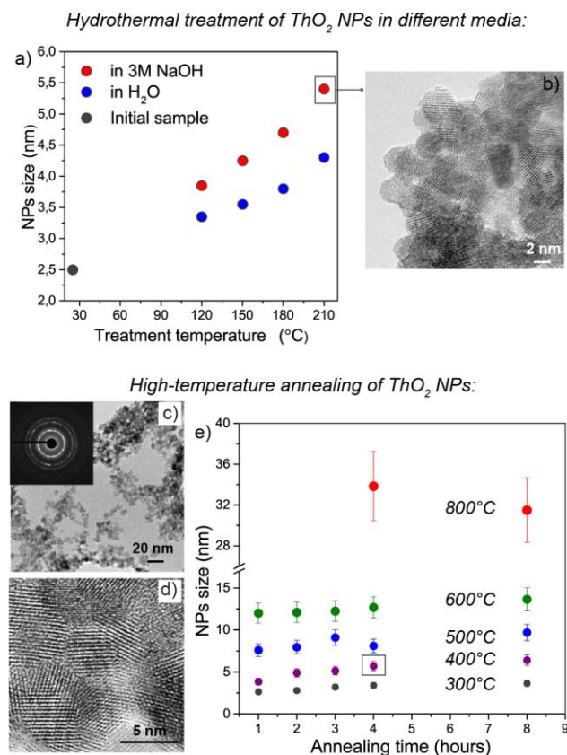
Fig. 2. a) Dependence of ThO 2 NPs size, as calculated from XRD data, on the temperature of hydrothermal treatment in different media. b) HRTEM data for ThO 2 sample treated hydrothermally at 210 °C in 3M NaOH. c), d) HRTEM and ED (insert) data for ThO 2 sample obtained by annealing thoria NPs at 400 °C for 4 hours. e) Size of ThO 2 NPs, as calculated from XRD data, vs. duration and temperature of annealing.
