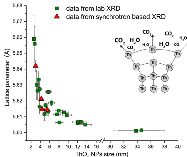
Fig. 4. ThO 2 unit cell parameter dependence on particle size. Insert: schematic representation of the lattice expansion mechanism
