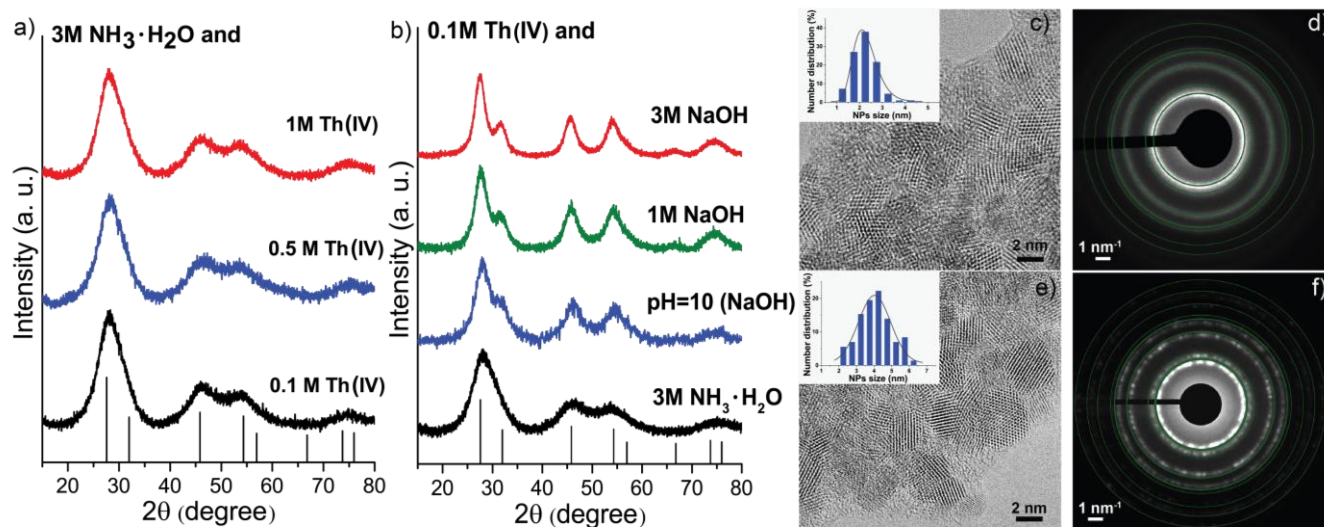
Fig. 1. a), b) XRD patterns of \text{ThO}_2 samples precipitated from thorium nitrate solutions of various concentrations (0.1M – 1M) using aqueous ammonia and NaOH aqueous solutions (1M and 3M) as precipitants. HRTEM and ED data for thoria NPs obtained by precipitation from 0.1 M \text{Th}(\text{NO}_3)_4 \cdot 5\text{H}_2\text{O} and c), d) 3M \text{NH}_3 \cdot \text{H}_2\text{O} ; e), f) 3M NaOH as precipitants. The circles on ED patterns indicate the diffraction pattern calculated for bulk \text{ThO}_2 24 . The inserts in HRTEM images show the size distributions of \text{ThO}_2 NPs, as obtained from HRTEM data.
