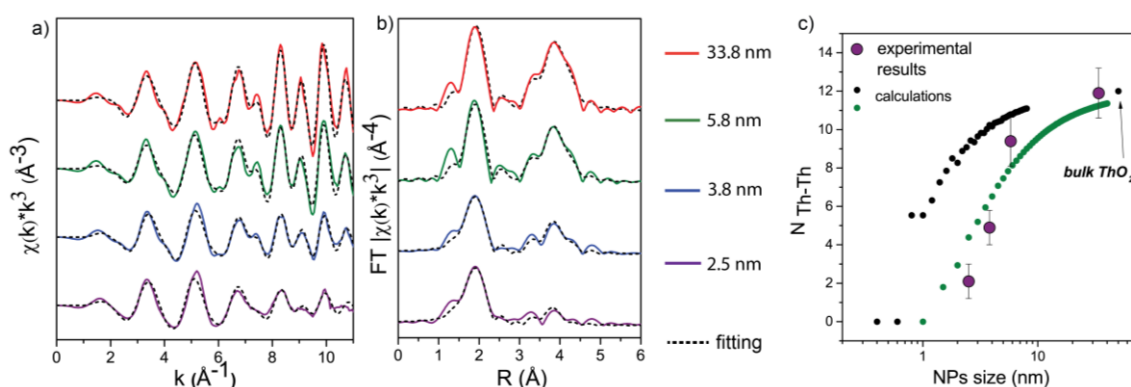
Fig. 3. Th L3-EXAFS R-space fitting results for 2.5, 3.8, 5.8 and 33.8 nm ThO 2 samples: a) k^3 -weighted \chi(k) experimental functions (coloured solid lines) and corresponding fitting models (dashed lines); b) FT magnitude of EXAFS data (coloured solid lines), fit magnitude (dashed lines); c) Comparison of the size-dependent change of Th-Th coordination number in ThO 2 NPs, as determined by EXAFS vs. calculated values for ThO 2 particles of different size; black dots correspond to value of Th atoms in the second coordination shell in spherical NPs with a ThO 2 crystal structure; green dots correspond to calculated effective Th-Th coordination number according to equation (2).
