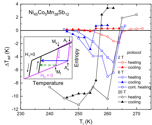
FIG. 4. Adiabatic temperature change of \text{Ni}_{45}\text{Co}_5\text{Mn}_{38}\text{Sb}_{12} around the martensitic transformation, obtained under magnetic field pulses of 2, 6, and 20 T following discontinuous heating (circles) and discontinuous cooling (triangles). For a field change of 6 T also continuous heating data were recorded (squares). Inset: schematic of the adiabatic cooling in case of using heating- (continuous blue arrow) or cooling- (discontinuous green arrow) protocol. See text for details.
