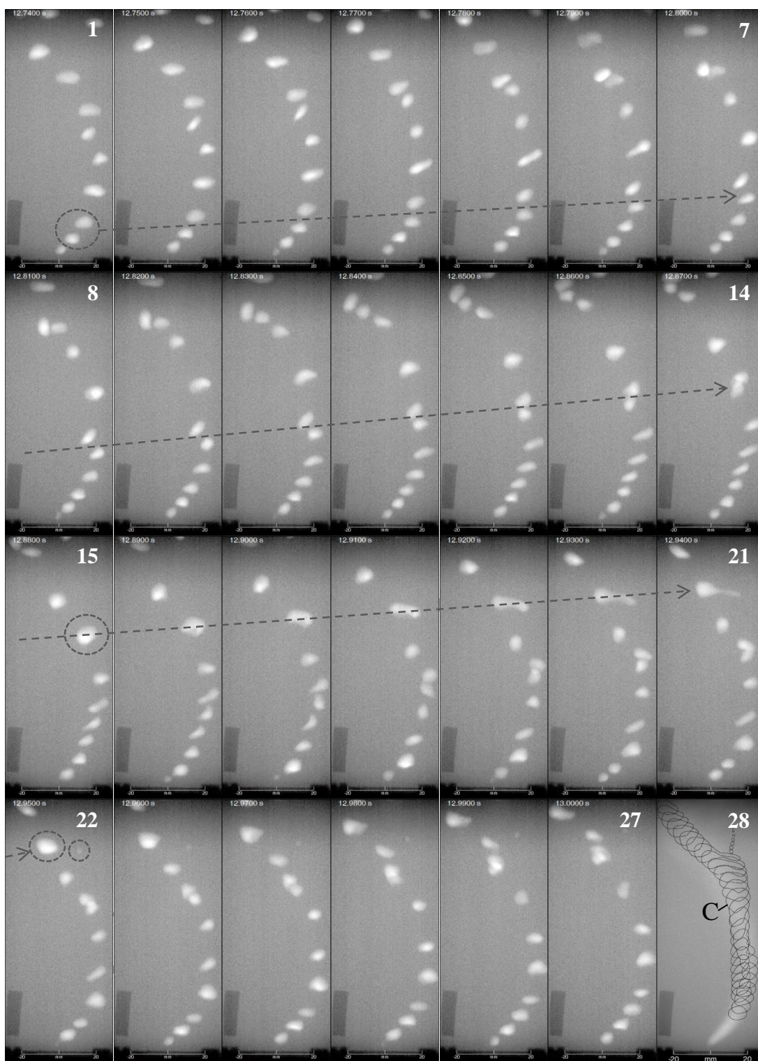
Figure 5. Sequence of single frames illustrating bubble coalescence with subsequent breakup initiated by stretching at a gas flow rate of 600 \text{ cm}^3/\text{min} . Time step between two frames is 0.01 \text{ s} . Frame 28: evolution of the bubble surface.
