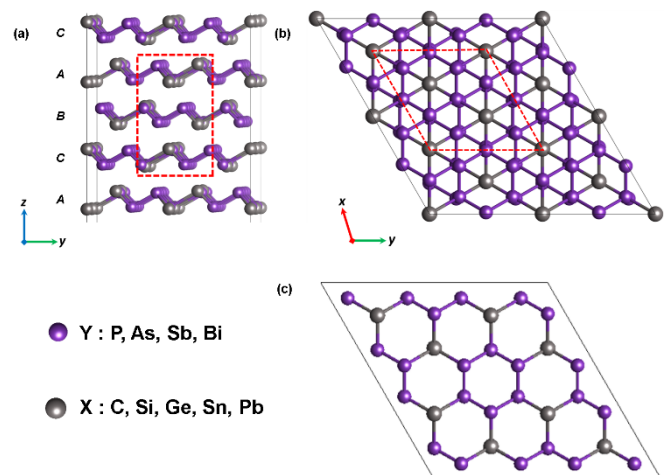
Figure 1 Crystal structures of bulk \text{XY}_3 systems in the 2 \times 2 \times 2 supercell representation: (a) side and (b) top views. Purple and grey represent Y and X atoms, respectively. (c) Top view of a \text{XY}_3 monolayer. Figures were created using 3D visualization package VESTA.[54]
