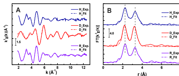
Figure 2. A). Ag K-edge of k^3 -weighted EXAFS function and B). Corresponding phase corrected Fourier Transform (FT) best fits of the sample in hydrated (H), dehydrated (D), and rehydrated (R) states. The experimental (Exp.) and fitted data are indicated with solid and broken lines to visualize the fitting quality.
