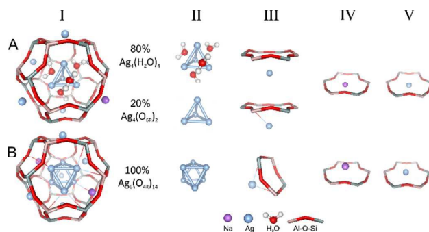
Figure 3. Schematic 3D structure of the AgCs and their surrounding environments inside the sodalite cage of sample in A). (re)hydrated and B). dehydrated state. The complete atomic structure of the sodalite cage embedding the AgCs including its extra-framework water ligands and the Ag and Na cations located in the S6Rs of the cage. (I), AgCs structural fraction that depicts the presence or absence of the water ligands. (II), the interaction of the AgCs atoms with the O_F of the sodalite S6Rs or S4Rs (III), the actual positions of Na (IV), and Ag cations (V) along the axis of the S6Rs.
