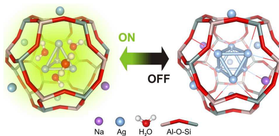
Figure 4. Schematic of reversible opto-structural switching of AgCs confined in \text{Ag}_3\text{Na}_9\text{LTA} sodalites.
