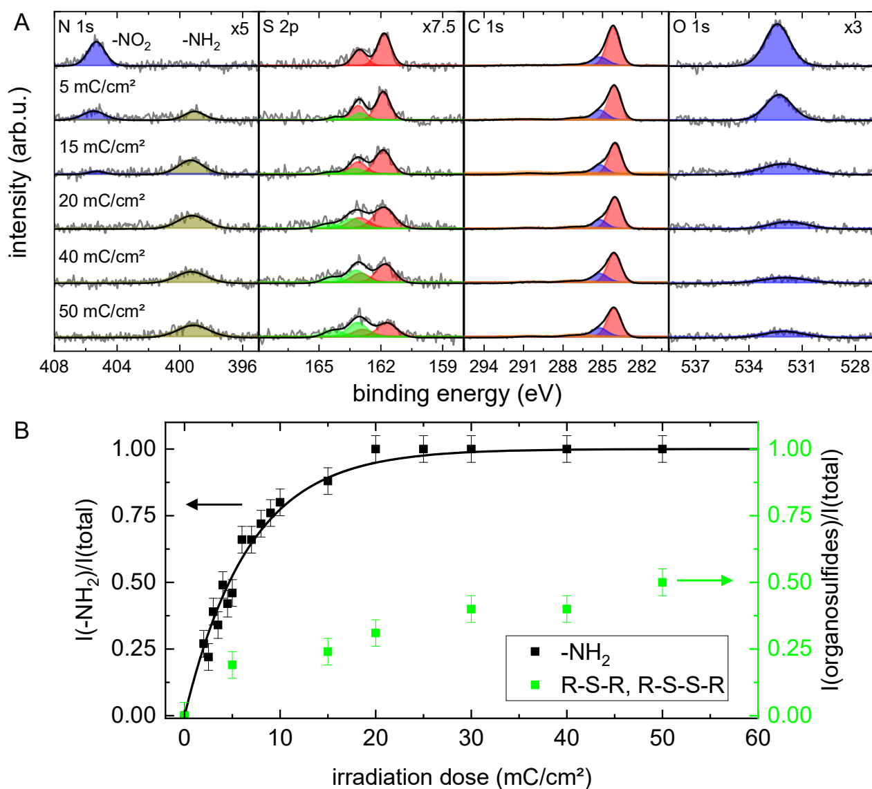
Figure 2: (A) N 1s, S 2p, C 1s and O 1s XP spectra of a NBPT SAM which is stepwise irradiated with electrons with an energy of 50 eV and subsequently crosslinked into a Carbon Nanomembrane. For better representation, intensities of the N 1s, S 2p and O 1s spectra are multiplied by the factor presented in the figure. (B) fraction of -NH 2 and organosulfide (R-S-R and R-S-S-R) groups, respectively, for different irradiation doses determined by the XPS results presented in (A)
