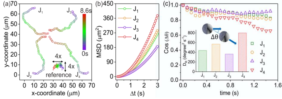
Figure 3. (a) Trajectories of four single Janus PS/Ag/AgCl particles (J 1 -J 4 ) taken over 8.6 s under blue light illumination [(106 ± 1) /mm 2 ]. The trajectory of a reference Janus PS/Ag/AgCl particles under green light illumination [(8 ± 1) μW /mm 2 ] is shown as well (video S1). (b) The experimental MSD curves of single Janus particles: J 1 (1193 μm 2 , green symbols), J 2 (1460 μm 2 , orange symbols), J 3 (940 μm 2 , purple symbols), and J 4 (2899 μm 2 , red symbols) (video S1). (c) Time evolution of the experimental autocorrelation values, Cos(Δθ), of the angle Δθ between two neighboring frames in the tracking video files for the single Janus PS/Ag/AgCl particles (J 1 -J 4 ). The upper inset shows schematics on how the angle Δθ is defined. The lower inset summarizes the rotational diffusion coefficients, D R , for four single Janus particles (video S2).
