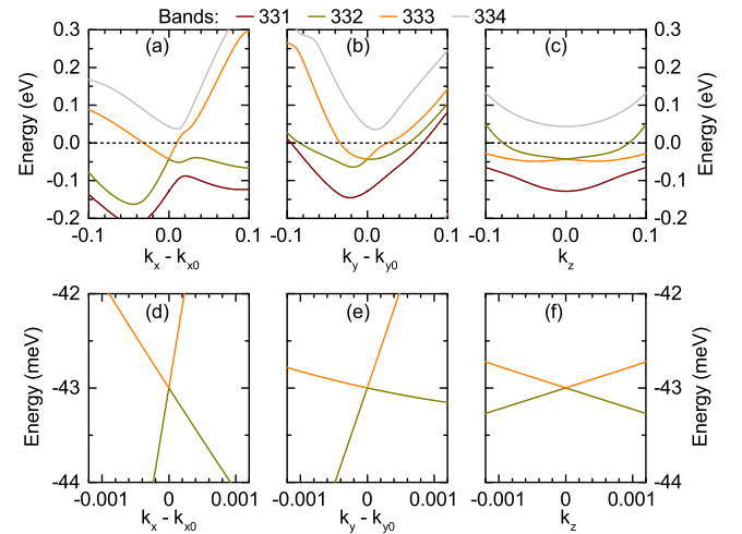
FIG. 6. Band structure of \alpha -PdBi in the vicinity of the Weyl node at \mathbf{k}_0 = (k_{x0}, k_{y0}, k_{z0}) = (0.399706, 0.056504, 0)2\pi/a . The cuts are running parallel to the (a) k_x , (b) k_y , and (c) k_z directions. The band colors are identical to those used in Fig. 5(a). (d), (e), and (f) are zooms into (a), (b), and (c), respectively. In these zoomed images, we used a fine k spacing of steps in the range |\mathbf{k} - \mathbf{k}_0| \leq 10^{-3} in order to show that the crossing is indeed nearly linear in all directions.
