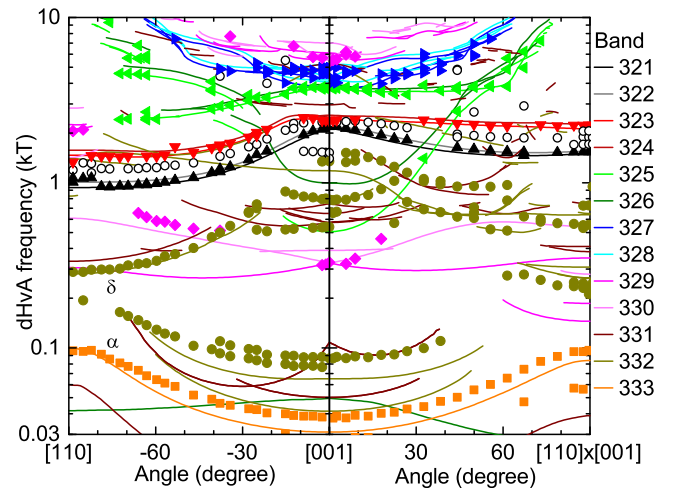
FIG. 4. Angular dependence of the experimentally observed dHvA frequencies (symbols) and of the calculated extremal Fermi-surface cross-sections (lines) in \alpha -PdBi. The line colors correspond to the band and FS colors shown in Fig. 5. Empty symbols denote frequencies which could not clearly be assigned to a calculated frequency branch. Since spin-split bands in \alpha -PdBi produce similar Fermi-surface sheets and, hence, similar dHvA frequencies, we assigned and color-coordinated the experimental data only to the pair of bands. \alpha and \delta label the frequency branches which were also observed by Khan et al. [26].
