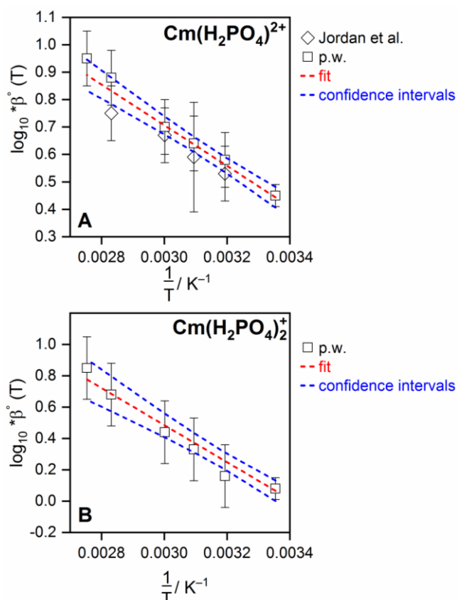
Figure 5: van't Hoff plots for the Cm(H 2 PO 4 ) 2 + (A) and Cm(H 2 PO 4 ) 2 + (B) complexes, based on the data in Table 5 and Table 6.
