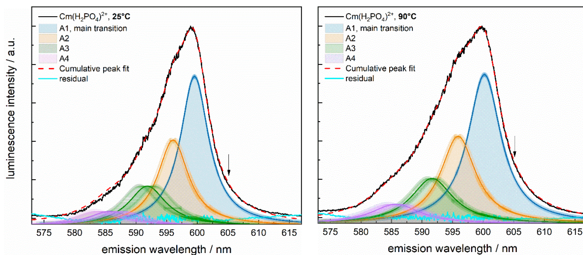
Figure 7: Extracted pure component emission spectra (black curves) of the Cm(H 2 PO 4 ) 2+ complex at 25 °C (left) and 90 °C (right) can be described with four Lorentzian peaks following the Boltzmann distribution depicting the emission transitions from the four crystal field states of the excited electronic level (A 1 –A 4 ) back to the ground state. Errors expressed with 99.7% (3σ) confidence of the fitted Lorentzian peak maxima and the fit residual (cyan traces) are included in the plots. Arrows indicate the part of the spectrum where the presence of an 8–fold coordinated Cm(H 2 PO 4 ) 2+ complex would be expected to appear.
