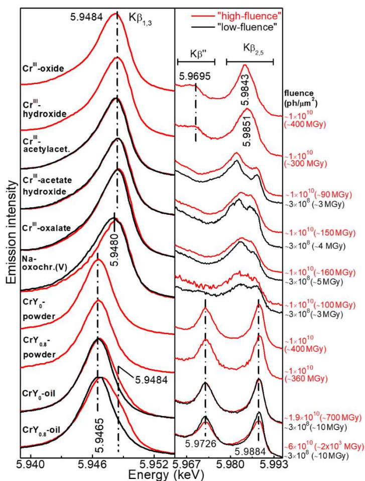
Figure 2. Cr-K \beta XES spectra of Cr-samples recorded using “high-fluence” (red) and “low-fluence” (black) conditions at ESRF-ID26: (left) K \beta 1,3 line; (right) K \beta satellite lines (see Figure S2 for the complete spectra of K \beta main lines). Fluences along with absorbed doses (in brackets) are also reported.
