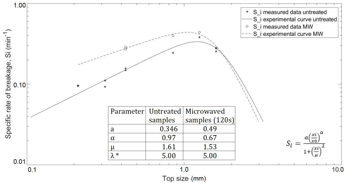
Figure 8. Specific rate of breakage for untreated and microwave-treated samples. (*) λ values are not deemed accurate as there is not enough data on coarser sizes to be able to quantify the deceleration rate
