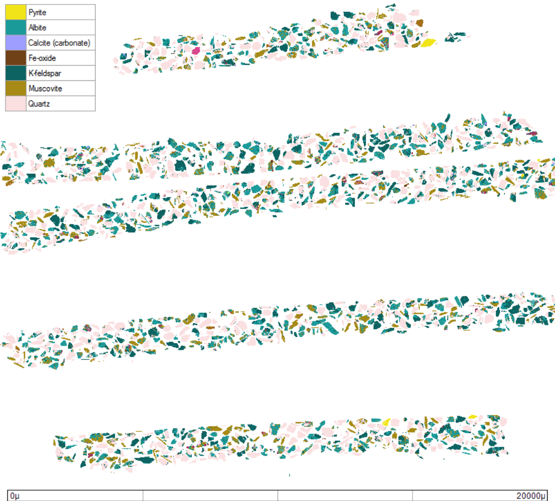
Figure 1. Mineral liberation analysis image from the feed sample (experiment on top size fraction -425+315 μm). 52 particles containing sulfide minerals (in yellow) were found in this sample (out of 5233 particles in total). Major minerals are shown in the legend
