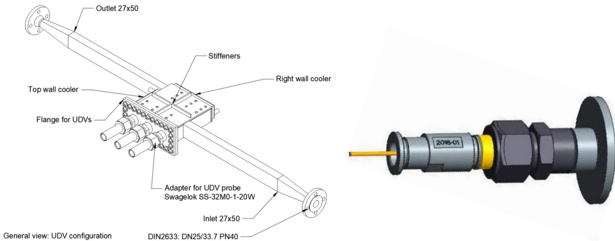
Figure 4: Left, final design of STS from KTH in configuration with UDVs from HZDR. Source: KTH. Right: UDV socket with installed transducer mounted at test section. Source: HZDR.
