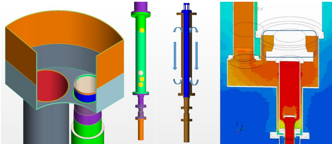
Figure 6: Illustration of small CIRCE improvement. Left, separator: in orange, added lateral wall. Centre, FPS lateral openings and possible buoyant recirculation pattern. Right: temperature in conveyor with indication of possible trapped gas region
