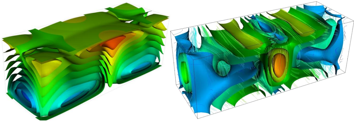
Figure 12: Reyleigh-Benard convection POD-Galerkin simulation. Left, first temperature mod. Right, first velocity mod. Source: KIT-IKET.
