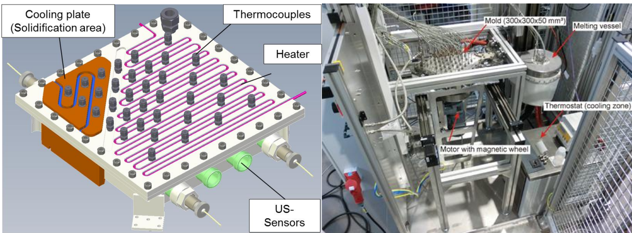
Figure 5: HZDR pool solidification facility for instrumentation testing. Left, pool design. Right, facility. Source: HZDR.
