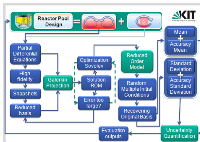
Figure 11: Conceptual sketch and contextualization of the POD-Galerkin approach. Source: KIT-IKET.
