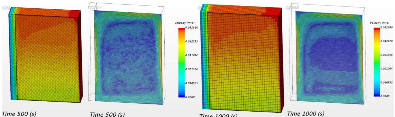
Figure 9: Buoyancy driven simplified test case. Temperature and flow with polyhedral mesh (left), with trimmed mesh (right)
