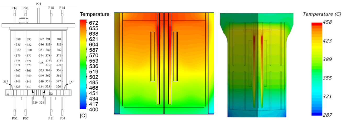
Figure 10: SESAME-stand from CVR. Experimental temperatures (left). Simulation without thermal radiation (center). Simulation with thermal radiation (right)
