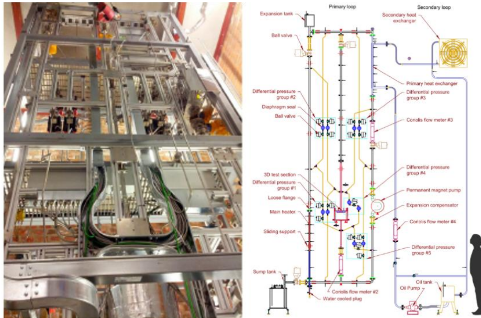
Figure 2: TALL-3D facility by KTH. Left, facility. Right, functional sketch. Source: KTH.
