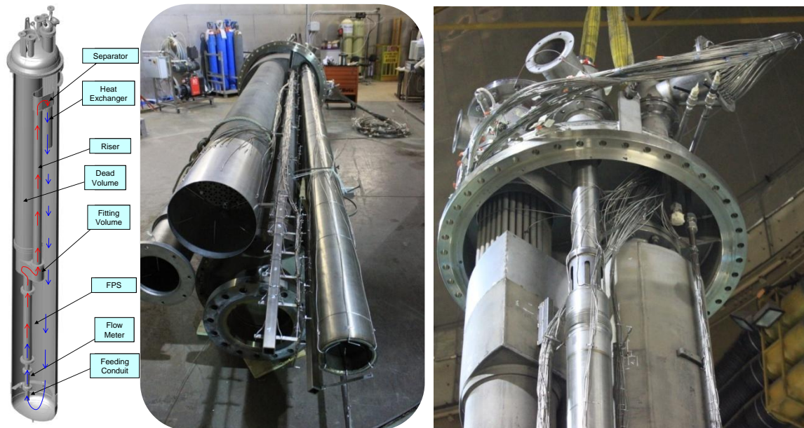
Figure 1: CIRCE facility from ENEA. Left, functional sketch. Components above the fitting volume (center) and at the top (right). Source: ENEA.
