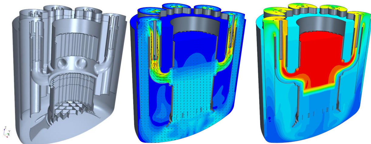
Figure 14: ALFRED according to LEADER project. Geometry (left). Velocity field (center). Temperature (right). Source: NRG.
