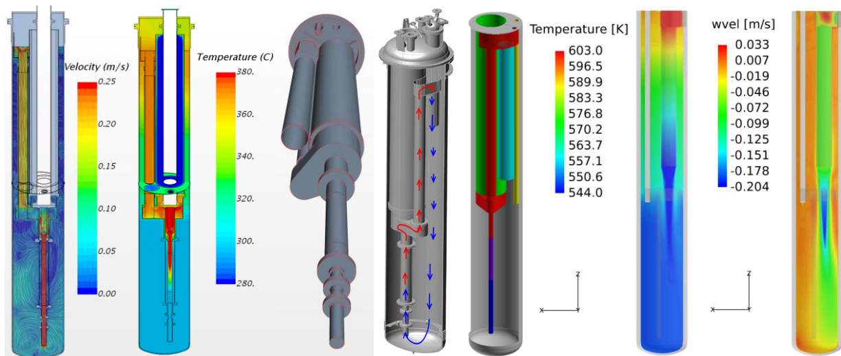
Figure 13: CIRCE representation. Centre, CAD from ENEA. Left, detailed CFD by CRS4. Right, simplified CFD by NRG.
