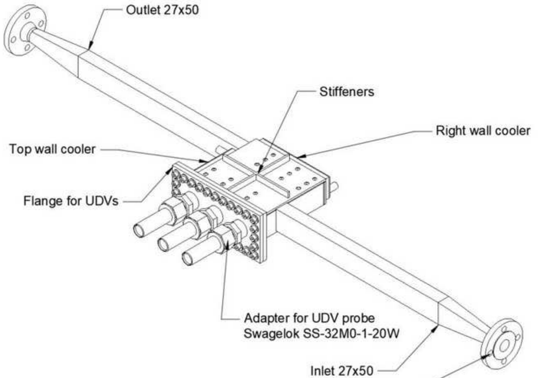
General view: UDV configuration
