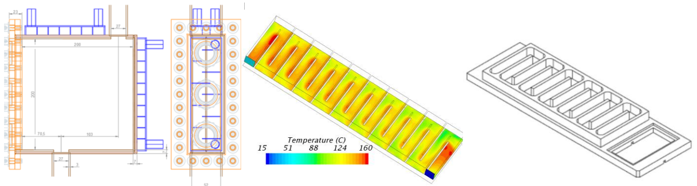
Figure 8: STS design with the water coolers leading to local boiling. Left, design. Centre, wall temperature. Right, improved design.
