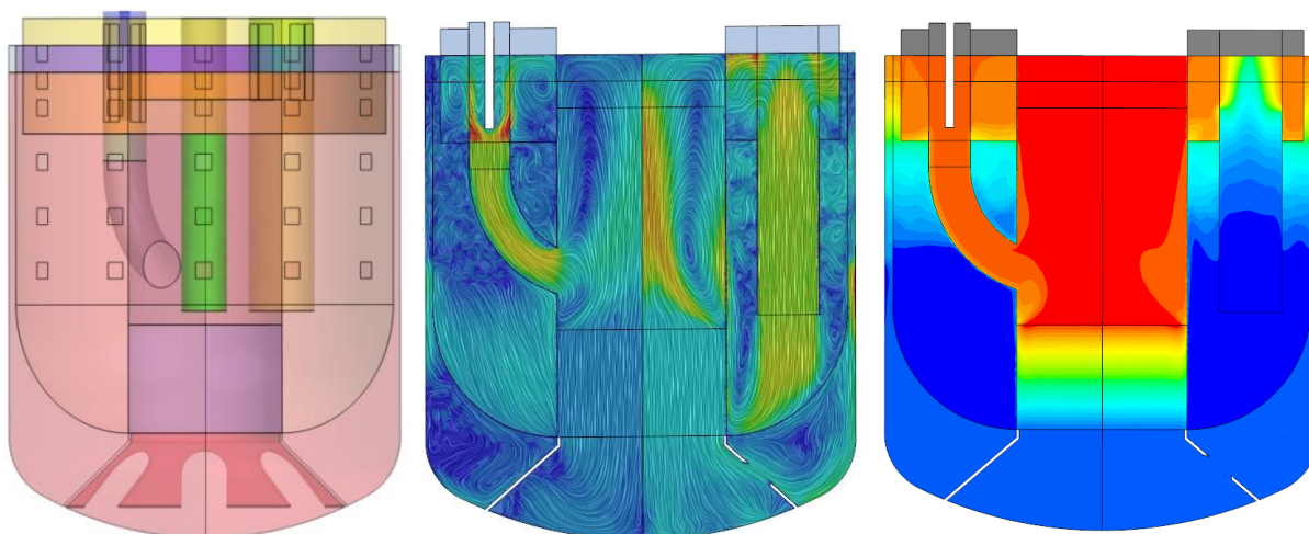
Figure 15: ALFRED according to Ansaldo design. Geometrical structure (left). Velocity field (center). Temperature (right)
