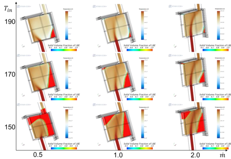
Figure 7: STS Pre-test parametric study performed by KTH: frozen fraction depending on inlet temperature and mass flow rate
