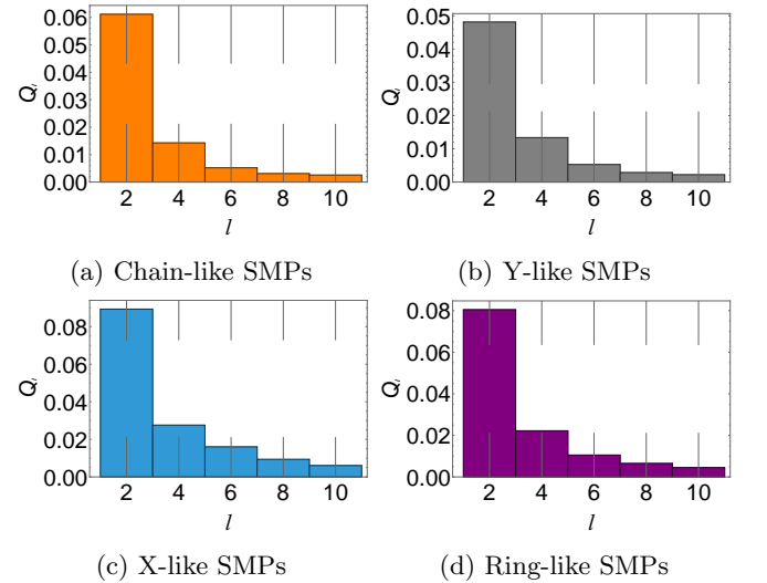
FIG. 11: Histograms of Q_l , Eq. (9). The values are averaged over all production runs. Subfigures are for clusters formed by (a) chain-like SMPs; (b) Y-like SMPs; (c) X-like SMPs and (d) by ring-like SMPs.
