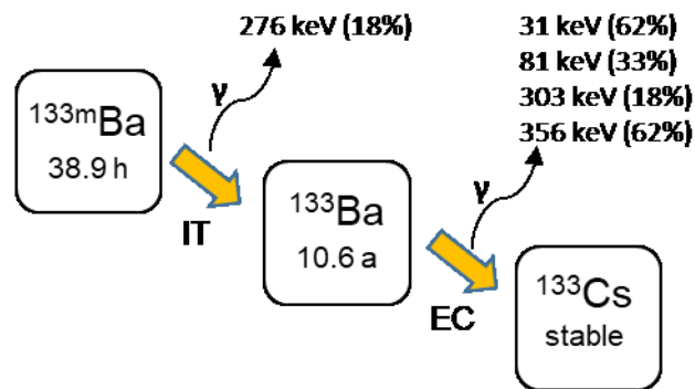
Figure 6. Decay scheme of metastable ^{133m}\text{Ba} over ^{133}\text{Ba} to stable ^{133}\text{Cs} .
