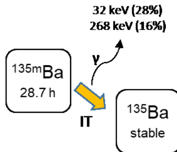
Figure 5. Decay scheme of metastable ^{135m}\text{Ba} to stable ^{135}\text{Ba} .
