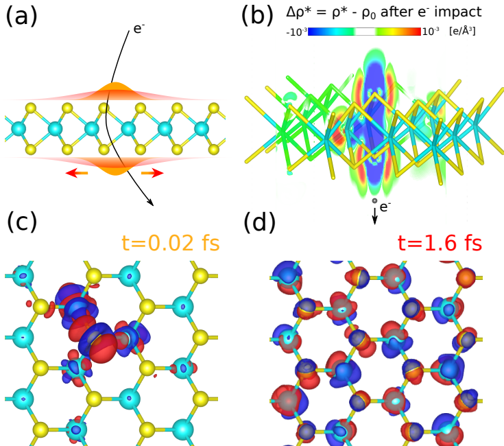
Figure 1: ED simulations of a high-energy electron impact into MoS 2 sheet. The electron is modeled as a classical particle with a precisely defined trajectory, which can give rise to electronic excitations in the target material, as schematically illustrated in (a). (b) The spatial extent of the electronic excitation created in the system immediately after the impact. (c) Simulations where exactly one electron is excited with the excitation initially being localized on a sulfur atom. (d) The spatial extent of the excitation after 1.6 fs as described within the framework of ED.
