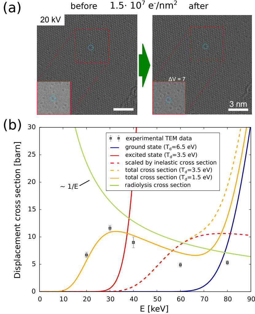
Figure 3: (a) Cc/Cs-corrected HRTEM images of single-layer MoS 2 before and after exposure to the total dose of 1.5 \cdot 10^7 electrons/nm 2 at an acceleration voltage of 20 kV. During irradiation, S vacancies appear. Fourier-filtered images from the red dashed framed area are given in the insets (solid frames). As an example, a vacancy in each filtered and raw image is marked by a cyan circle. \Delta V gives the number of the produced vacancies. (b) The experimental (squares) and theoretical (curves) displacement cross sections \sigma of S atoms in MoS 2 , as calculated within the framework of the McKinley-Feshbach formalism with account for thermal vibrations and with different values of displacement threshold T_d , corresponding to the ground and excited states. The decrease in the excitation probability with increasing electron energy is accounted for within the framework of the Bethe theory. The total cross section with a T_d = 1.5 \text{ eV} , which matches the experimental data reasonably well is also shown.
