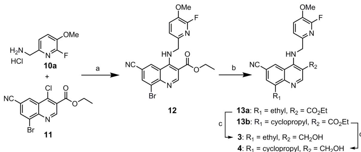
Scheme 1. Synthesis of "north region" compounds 3 and 4 .
