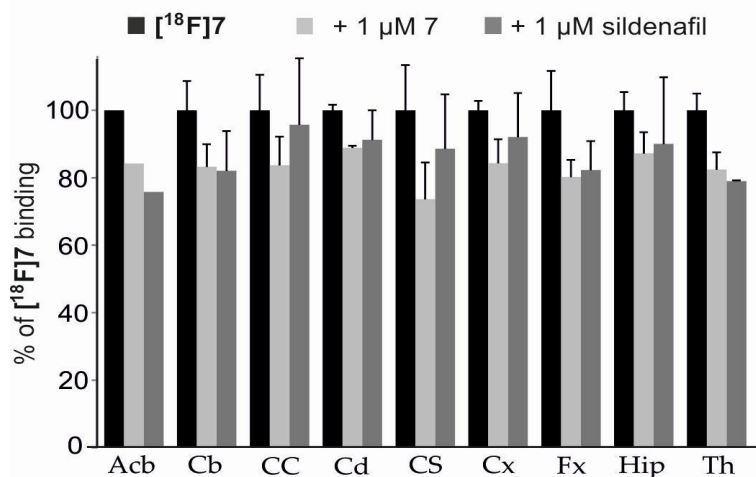
Figure 2. Binding of [ ^{18}\text{F} ]7 ( 2.02 \pm 0.75 nM) in porcine brain in vitro (n=3). Remaining binding of [ ^{18}\text{F} ]7 in the presence of 1 \mu\text{M} 7 or 1 \mu\text{M} sildenafil is presented as percentage of total binding (= 100%). Abbreviations: Acb = Nucleus accumbens, Cb = Cerebellum, CC = Corpus callosum, Cd = Nucleus caudatus, CS = Colliculus superior, Cx = Cortex, Fx = Fornix, Hip = Hippocampus, Th = Thalamus.
