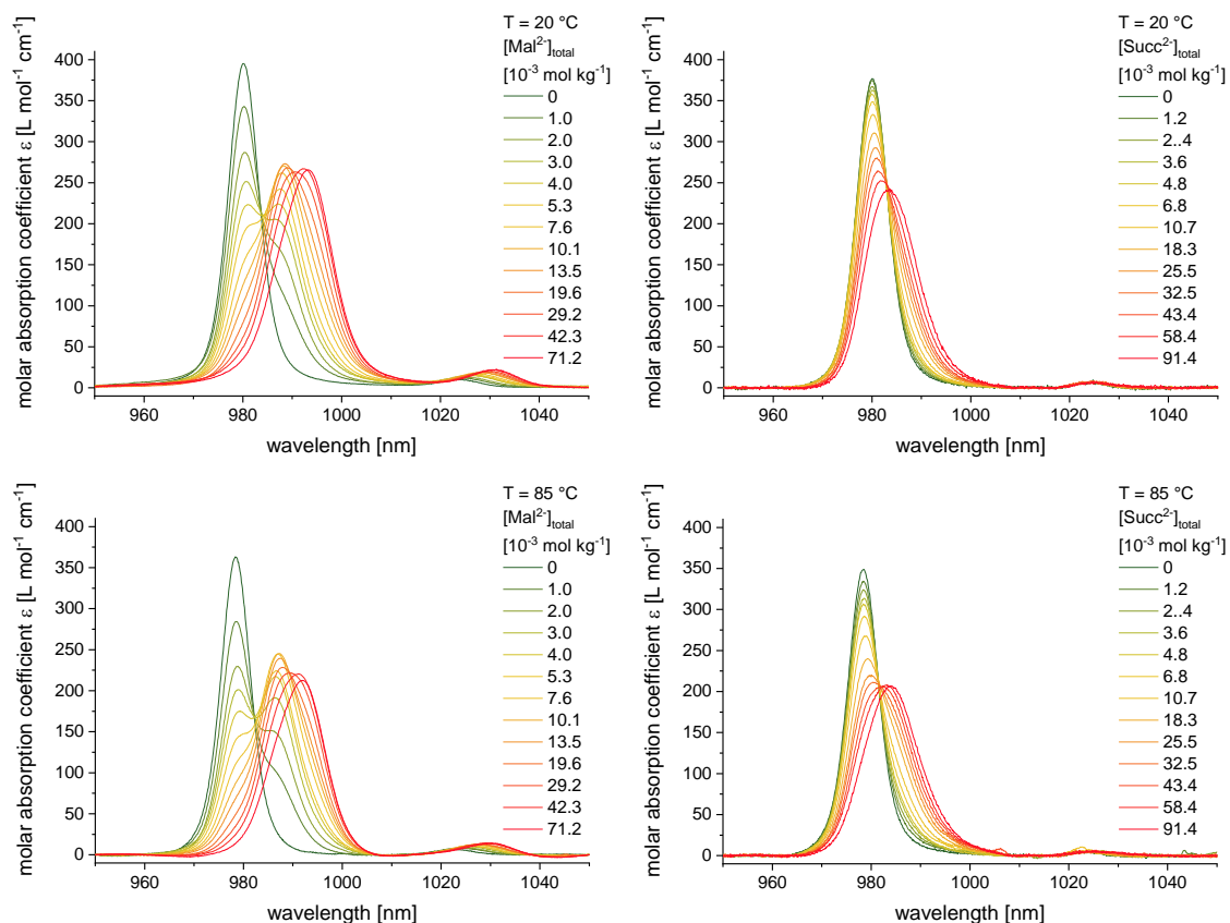
Figure 1: Absorption spectra of Np(V) with increasing malonate (left) and succinate (right) concentration at T = 20 (top) and 85 °C (bottom) and I_m(\text{NaClO}_4) = 1.0 mol kg -1 .
