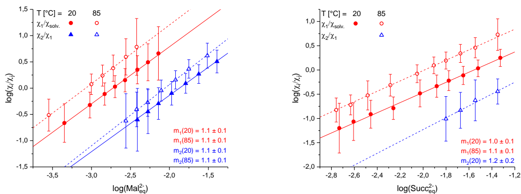
Figure 4: Plots of \log ([\text{NpO}_2(\text{L})_n]^{1-2n}/[\text{NpO}_2(\text{L})_{n-1}]^{3-2n}) vs. \log ([\text{L}^{2-}]_{\text{eq}}) and linear regression analyses at T = 20, 85 °C and I_m = 1.0 mol \text{kg}^{-1} \text{H}_2\text{O} . (left): \text{L}^{2-} = \text{Mal}^{2-} , (right) \text{L}^{2-} = \text{Succ}^{2-} .
