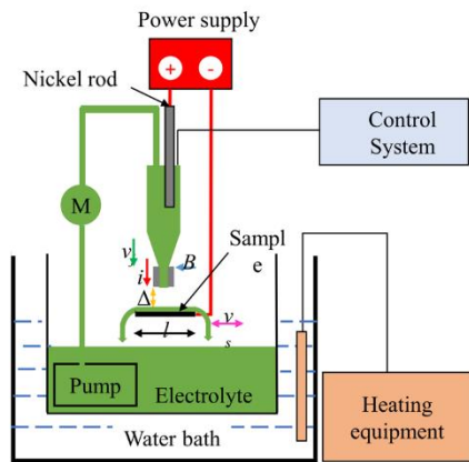
(a) System diagram of the magnetic-field-assisted jet plating
