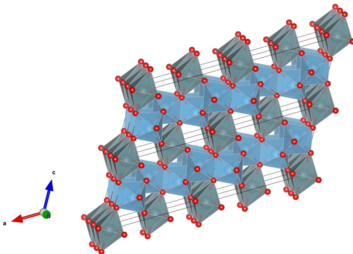
Figure 6: A polyhedral representation of the \text{UTi}_2\text{O}_6 brannerite structure, as reported by Szymanski and Scott 36 , with (\text{AO}_6) octahedra in grey, (\text{BO}_6) octahedra in light blue, and O atoms in red. The diagram shows a 2 \times 2 \times 2 unit cell ensemble. Produced in the VESTA software package 38 .
