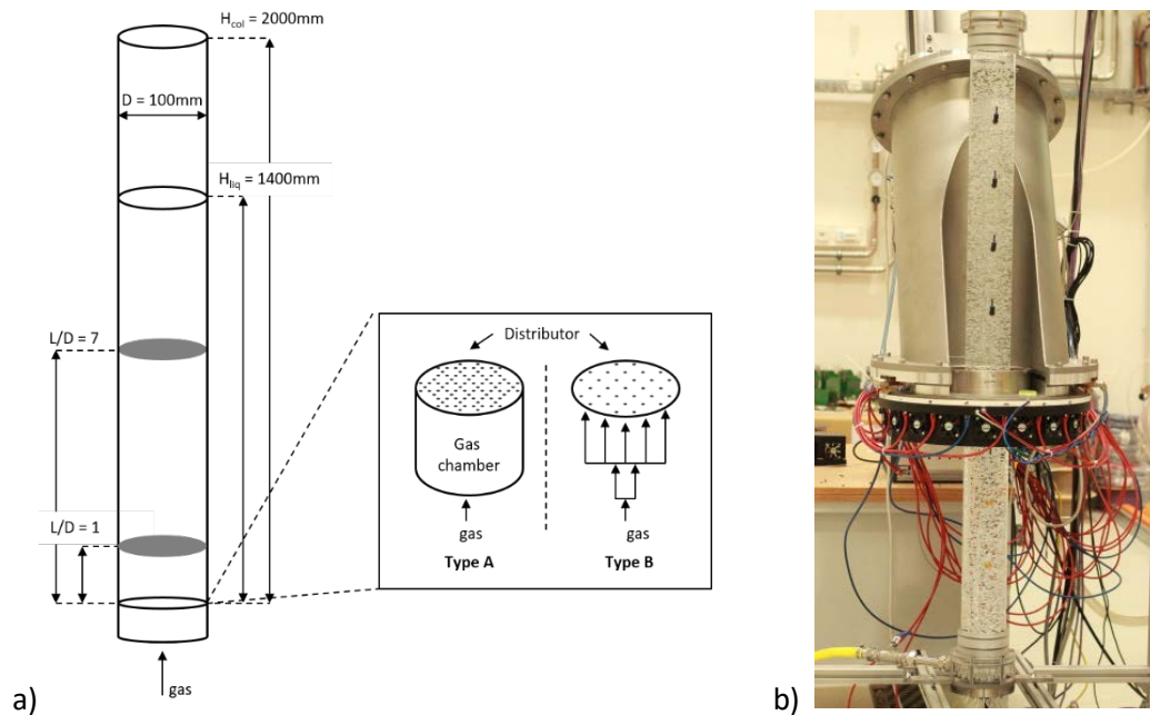
Figure 1: a) Schematic and b) photograph of the bubble column in the X-ray scanner.
