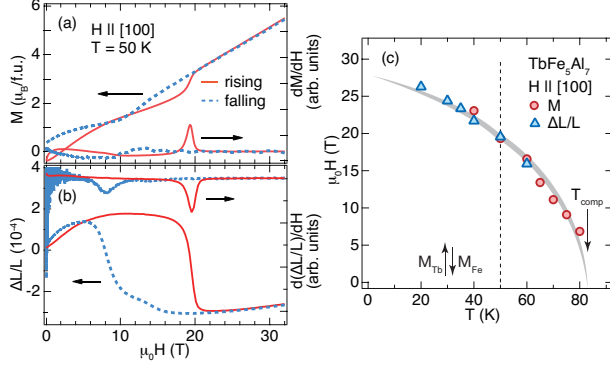
FIG. 3: (a) Magnetization and (b) longitudinal magnetostriction \Delta L/L (left scale) and its field derivative (right scale) at 50 K as function of magnetic field applied along the [100] axis. (c) H - T phase diagram of \text{TbFe}_5\text{Al}_7 with magnetic field applied along the [100] axis determined by peak positions in dM/dH and d(\Delta L/L)/dH data taken during field upswEEP. The gray solid line is a guide for the eyes. Soft x-ray spectra in pulsed magnetic fields, shown in Figs. 4, 5, and 6, were measured along the dashed vertical line. The antiparallel arrows sketch the collinear ferrimagnetic structure below T_{\text{comp}} .
