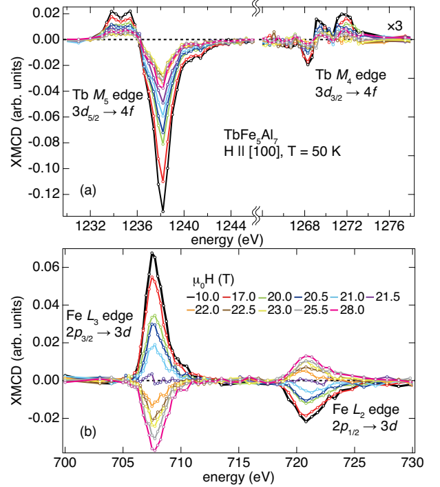
FIG. 4: (a) Tb M -edge and (b) Fe L -edge XMCD spectra at selected magnetic fields during the up sweep in pulsed magnetic fields at 50 K. All spectra are normalized to the (a) M -edge and (b) L -edge XAS integral at each field.
