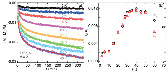
FIG. 2: (a) Time dependence of remnant magnetization (symbols) at selected temperatures after removing the cooling magnetic field of 14 T. The solid line is the fit of the double exponential function to the time evolution of magnetization at 40 K. (b) Relative amplitude of each exponential component, defined by Eq. (1), as a function of temperature.
