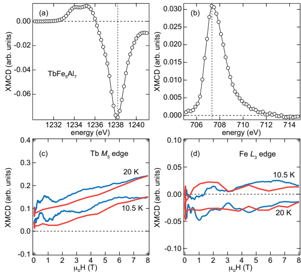
FIG. 1: XMCD spectra at the (a) Tb M_5 and (b) Fe L_3 edge. These spectra were obtained in zero field at 20 K after a field pulse of 10 T was applied along the [100] axis. The vertical dashed lines represent the photon energies at which magnetic-field-dependent XMCD data of (c) Tb and (d) Fe at 20 K and 10.5 K were recorded. The spectra are normalized to the XAS intensity at each energy and temperature. The sign of the XMCD in (c) and (d) is reversed with respect to those in (a) and (b). The positive (negative) values of the reversed Tb M_5 - and Fe L_3 -edge XMCD signals correspond to the moment direction (anti)parallel to the field direction.
