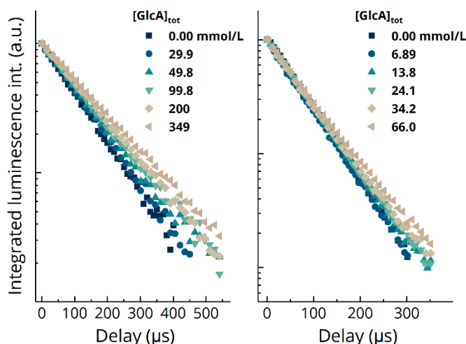
Figure 2: Luminescence decay profiles of Eu(III) (left) and Cm(III) (right) as a function of [GlcA]_{tot} at I_m(NaCl) = 0.919 and 0.911 mol kg -1 H 2 O, respectively.
