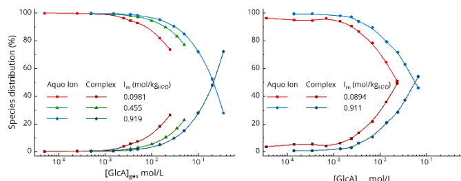
Figure 3: Speciation of Eu(III) (left) and Cm(III) (right) as a function of [GlcA]_{tot} at various I_m determined from TRLFS. The relative contribution of the aquo ion is displayed in light colors, the GlcA-complex in dark colors. The lines are guides-to-the-eye.
