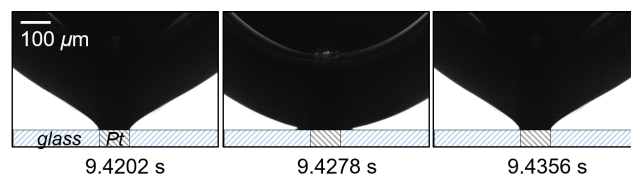
Fig. 10 Beyond Regime III ( 1 \text{ mol L}^{-1} at -12 V): Vertical oscillations in shape at high potential. The snapshots show the bubble in its upper, lower and again upper position shortly before detachment. Time counts from nucleation. The lifetime in this particular case is T = 9.4360 s. Image recording at 5380 frames/s. The potential is vs. MSE.
