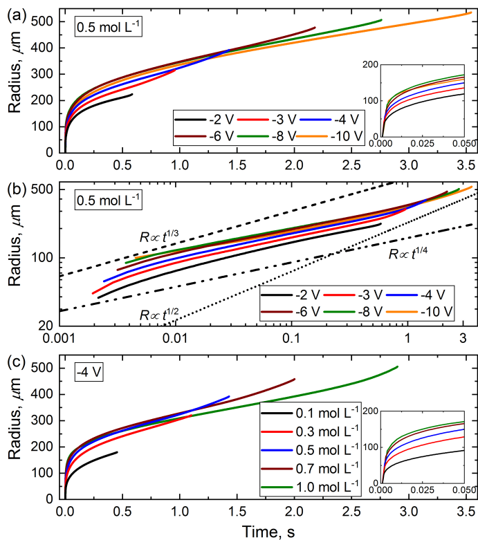
Fig. 4 (a) R(t) for different potentials and an electrolyte concentration of 0.5 \text{ mol L}^{-1} . (b) R(t) from (a), reproduced in double logarithmic scale. (c) R(t) for different electrolyte concentrations at a fixed potential of -4 \text{ V} . Each line starts from nucleation and ends at the detachment, and is the result of averaging over 8 bubbles. The insets show the initial phase of the bubble evolution. The potential is given vs. pseudo RE (Pt wire).
