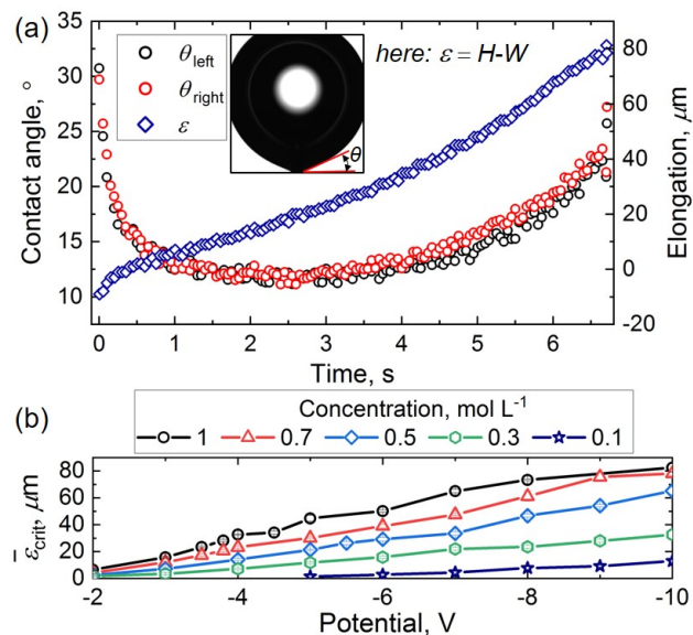
Fig. 9 (a) Variation in contact angle and elongation over time during one bubble cycle in Regime III ( 1 \text{ mol L}^{-1} at -10 V). (b) Critical elongation \bar{\varepsilon}_{crit} before the bubble detaches vs. potential at various concentrations. Each point represents a value averaged over 5...8 bubbles. The potential is vs. pseudo RE (Pt wire).
