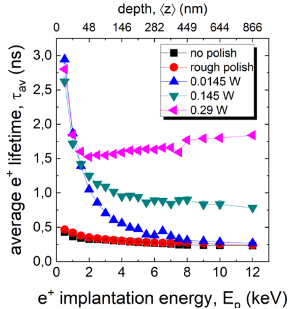
Figure 5: Average positron lifetimes for fs laser Si wafers, obtained from PALS.
