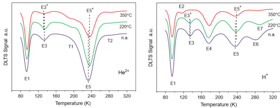
Figure 11 Majority carrier DLTS spectra of P + PN - N + diode measured after (a) He + irradiation and (b) H +
