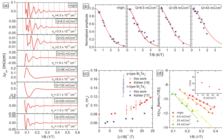
Figure 4 (Color online) (a) Oscillating part of the resistivity \Delta\rho_{xx} at 1.9 K for B \parallel c as a function of inverse magnetic field 1/B for different irradiation doses. (b) Temperature dependence of the oscillation amplitude with solid lines representing the fits obtained using the equation of \Delta\rho_{xx} \left( \frac{T}{B} \right) = \frac{\alpha T}{B \sinh(\alpha T/B)} . Different symbols correspond to the analysis of different Landau levels, i.e., peaks at different 1/B positions. In order to compare the temperature dependence of different peaks, the oscillation amplitudes have been normalized to the value of the fit for 1/B \rightarrow 0 . (c) Cyclotron masses m_c as function of the inverse oscillation period [\Delta(1/B)]^{-1} . (d) Dingle plots at T = 1.9 K and inset showing the mean free path l as a function of irradiation dose Q 32 .
