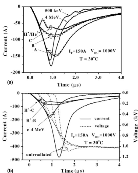
Figure 12 (a) Current reverse recovery characteristics of diodes irradiated by 500 keV ( 3 \times 10^{14} \text{ cm}^{-2} ) and 4 MeV ( 2 \times 10^{13} \text{ cm}^{-2} ) electrons (solid thin) and \text{H}^+/\text{He}^{2+} ions (fluence 5 \times 10^{12} / 5 \times 10^{11} \text{ cm}^{-2} , thick solid/dashed); (b) current (solid) and voltage (dashed) reverse recovery characteristics of the unirradiated diode and diodes irradiated by 4 MeV ( 2 \times 10^{13} \text{ cm}^{-2} ) electrons and \text{H}^+ ions (fluence 5 \times 10^{12} \text{ cm}^{-2} ). 73
