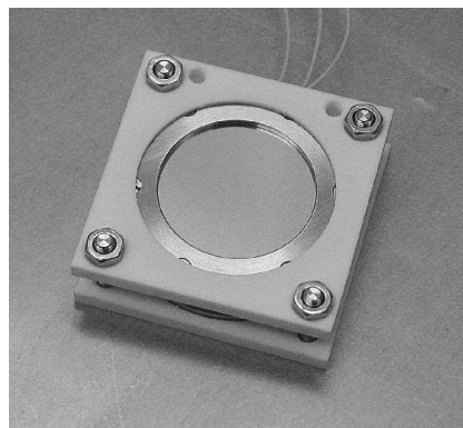
Fig. 2 The assembled monitor (electrode planes embedded in VITRONIT spacers).
