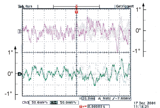
Fig. 3 Signal of the phase detector output for open loop for cavity 1 (top) and cavity 2 (bottom).
