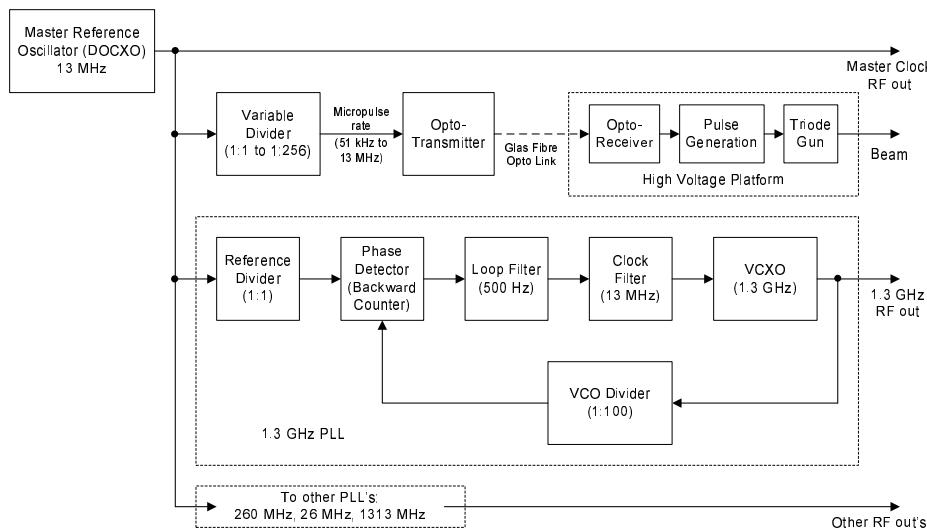
Fig. 1 Frequency generation for ELBE.
