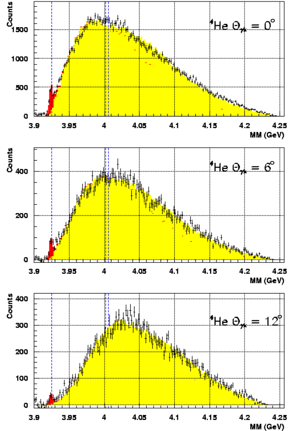
Fig. 2 Combined fit of quasifree missing mass distributions for ^4He(e, e'K^+) (yellow) and a ^4_\Lambda H bound state (red). The evidence is strong for all measured angles \theta_{\gamma K}^{lab} = 0, 6, 12 deg (i.e. also at higher momentum transfer t ). The dashed lines indicate the quasifree thresholds for \Lambda t , \Sigma^0 t , and \Sigma^- ^3He .
