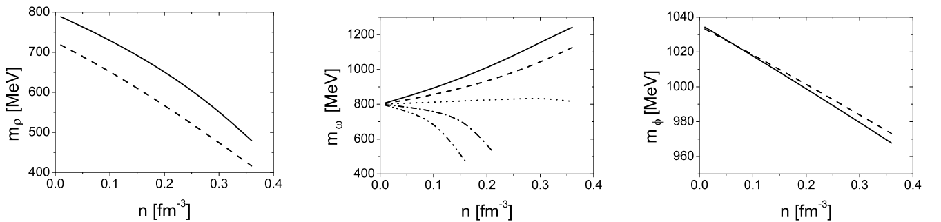
Fig. 1 The \rho, \omega, \phi meson masses as a function of the density. Full (dashed) curves in the left and right panels are for T = 20 (140) MeV. In the middle panel we have chosen T = 20 MeV and the various curves are for \kappa_N = 0 \dots 4 (from top to bottom), where the density dependence controlling parameter \kappa_N appears in the four-quark condensate q_4 = -\kappa_0 \langle \bar{u}u \rangle_0^2 \left[ 1 - \frac{\kappa_N}{\kappa_0} \frac{4M_N \sigma_N}{m_q \langle -\bar{u}u \rangle_0} I_1^N \right] entering the coefficient C_3 . \kappa_0 controls the vacuum saturation of the chiral condensate \langle \bar{u}u \rangle_0 , \sigma_N denotes the nucleon sigma term, and M_N is the vacuum nucleon mass; the term I_1^N depends on density and temperature, cf. [1].
