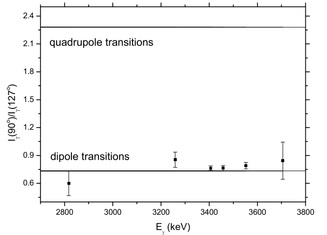
Fig. 2 Ratio of the \gamma -ray intensities observed at 90^\circ and 127^\circ . The theoretical values for pure dipole and quadrupole photons scattered from even-even nuclei are 0.734 and 2.28, respectively.
