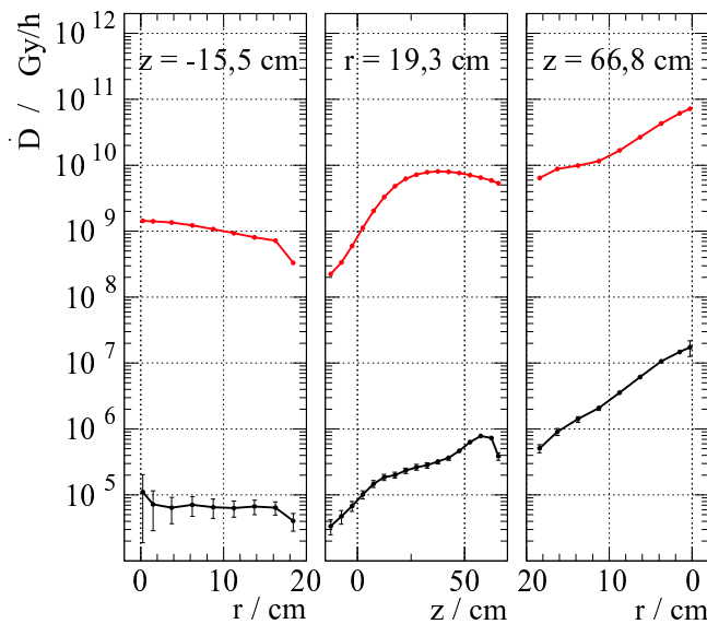
Fig. 2 Dose rate distribution near the steel vessel for a beam energy of 20 MeV and a current of 1 mA. The abscissa follow a closed path along the surface of the vessel. The photon dose rate exceeds the neutron dose rate by about 4 orders of magnitude.
