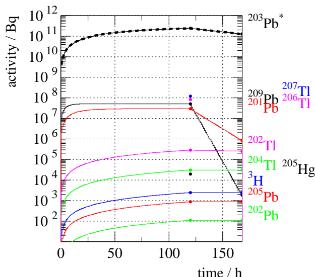
Fig. 2 The same as Fig. 1 but for radio-nuclides produced in the liquid lead; * activity is scaled by a factor F_c = 70 .
