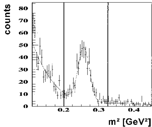
Fig. 2 Raw mass spectrum obtained for B = -1.4 T at \Theta_{lab} = 48^\circ . The peak in the range \Delta m^2 = 0.2 - 0.32 ( \text{GeV}/c^2 ) 2 is due to antikaons.
