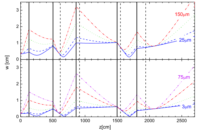
Fig. 2 Envelopes of the beam to laboratory 113a/b calculated for the beam of the U27 undulator with a 3 mm resonator hole (lower part, wavelength: 3, 10, 25, 50, 75 \mu\text{m} ) and for the U50 undulator with a 6 mm hole (upper part, wavelength: 25, 50, 100, 150 \mu\text{m} ). Additionally the positions of the mirrors are indicated by vertical lines (solid lines: focussing mirrors, dashed lines: plane mirrors).
