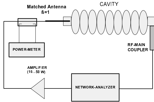
Fig. 2 Test setup.
