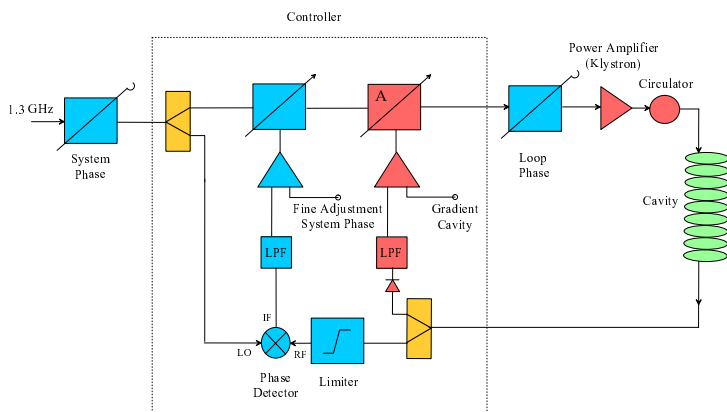
Fig. 2: Control loop design for amplitude and phase.
