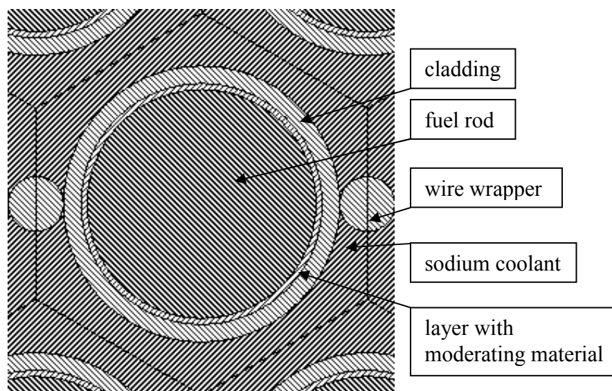
Fig. 1: Unit cell out of a fuel element based on the European fast reactor (EFR) design
