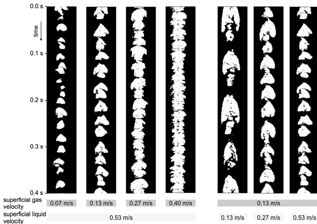
Fig. 3: Axial cuts of the reconstructed phase distributions at different gas and liquid flow rates
