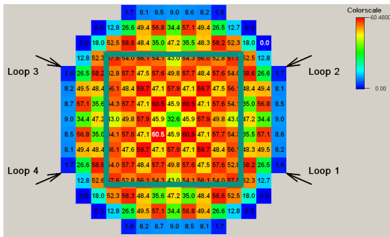
Fig. 2: Temperature differences at the core outlet for each fuel element position
