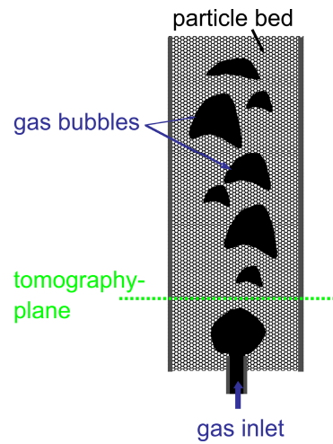
Fig. 4: Schematic of fluidized bed setup
