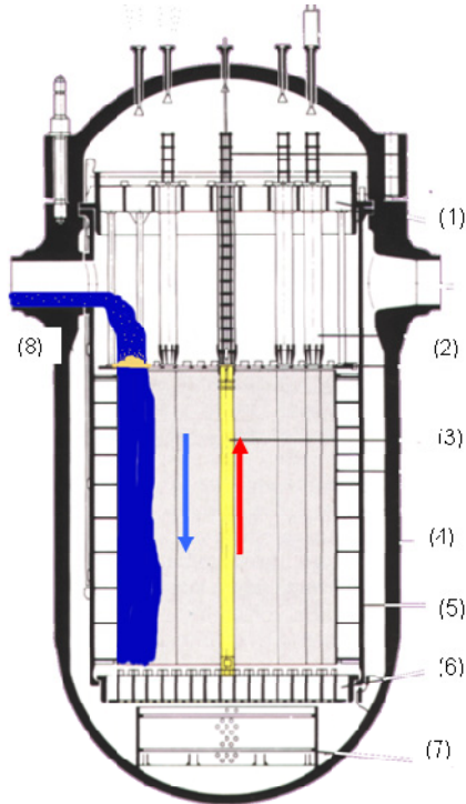
Fig. 1: RPV with ECC injection
