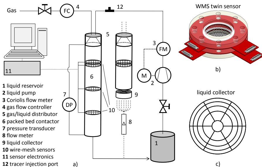
Fig. 1: Experimental contactor setup with WMS twin sensor and liquid collector
