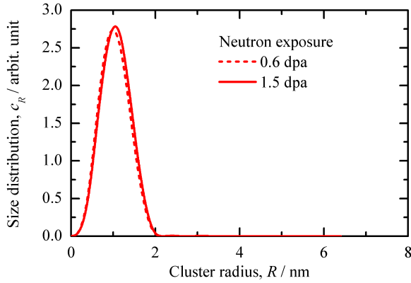
Fig. 3: Particle volume size distribution functions of irradiation-induced scatterers
