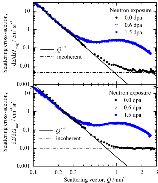
Fig. 1: Magnetic and nuclear scattering cross sections measured for the unirradiated control sample and two irradiated conditions of Fe-12.5at%Cr
