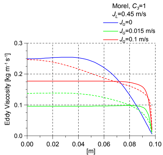
Fig. 7: Profiles for turbulent viscosity
