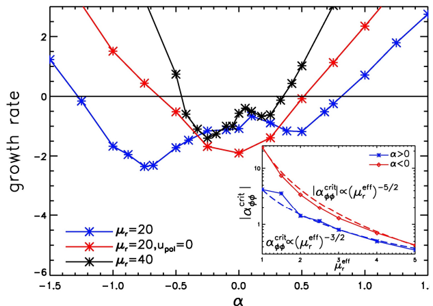
Fig. 7: Growth rates of the axisymmetric mode for Rm=30 in dependence on a prescribed homogenous \alpha -effect. In all cases the ( m=1 )-mode lies below the growth rates of the axisymmetric solution.
