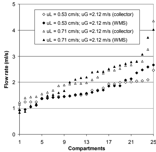
Fig. 5: Comparison of compartments flow rates from collector and wire-mesh sensor (sorted by increasing flow rate)
