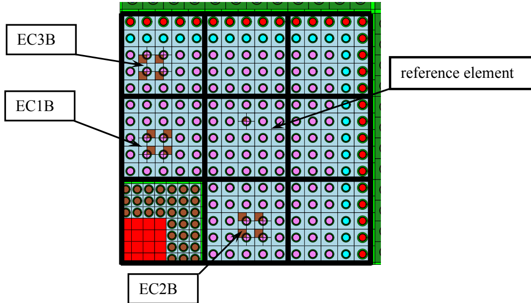
Fig. 1: Central fast area of the YALINA-booster core
