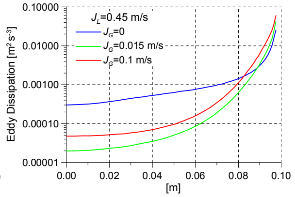
Fig. 2: Calculated profiles for the eddy dissipation
