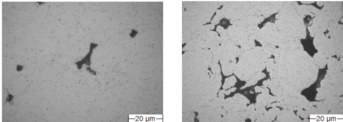
Fig. 3: Polished sections for ODS0.3A10 (left) and FeCr20 (right)
