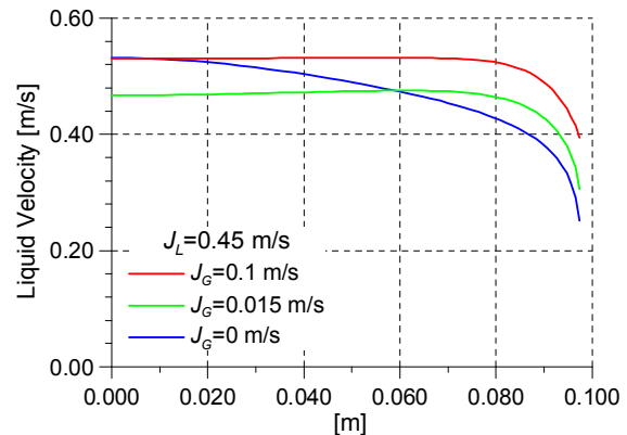
Fig. 4: Calculated profiles for the liquid velocity
