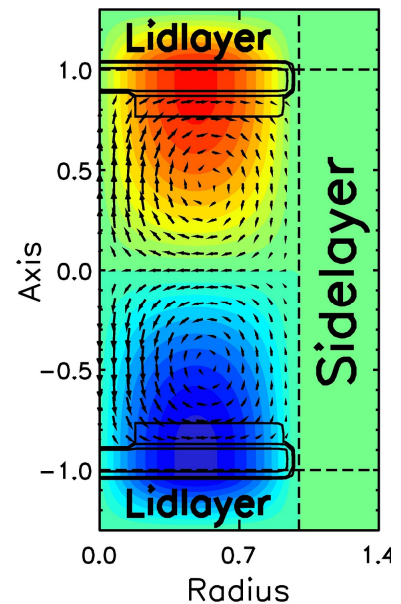
Fig. 3: Structure of the prescribed axisymmetric velocity field. The color coded pattern represents the azimuthal velocity and the arrows show the poloidal velocity field. The black solid lines represent the shape of the impeller system (disk and blades)
