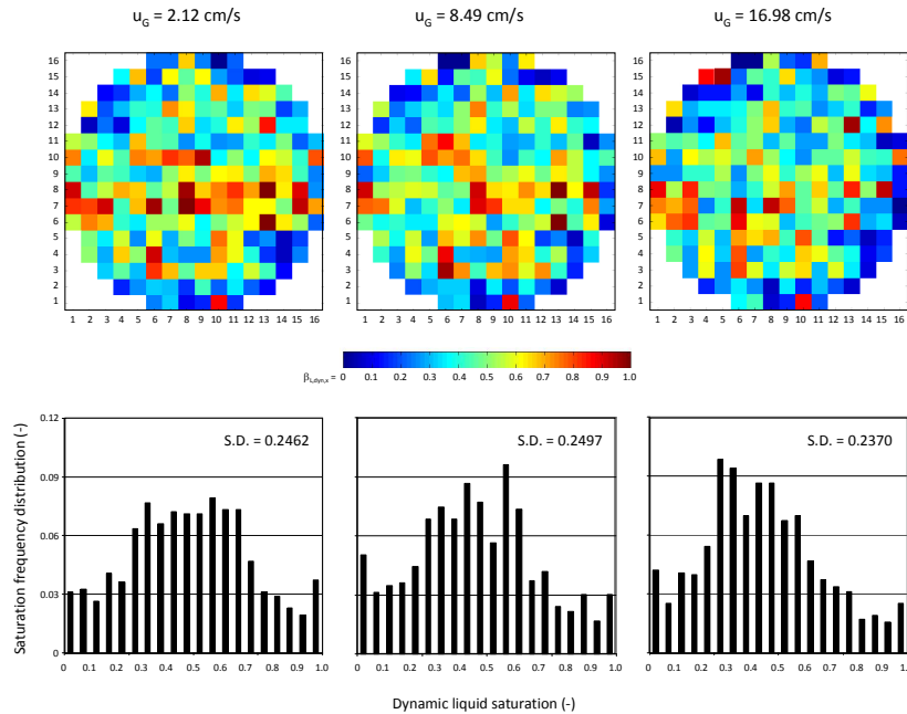
Fig. 3: Effect of superficial gas velocity on dynamic liquid saturation and corresponding frequency distribution of the local dynamic liquid saturation ( u_L = 0.53 \text{ cm/s} )
