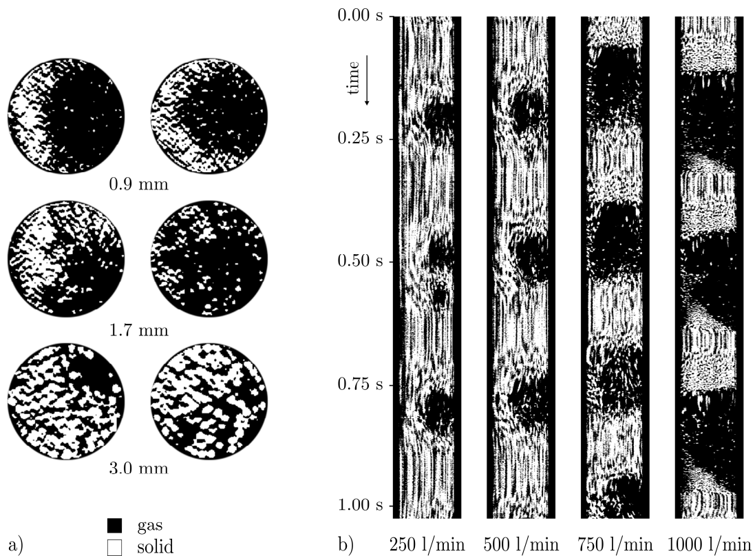
Fig. 5: Reconstructed phase distributions of the gas-solid two-phase flow in a fluidized bed: a) cross-sectional images for different particle sizes, b) axial cuts through the sequences with 1.7 mm spheres at different gas flow rates
