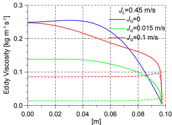
Fig. 3: Calculated profiles for turbulent eddy viscosity, the dotted lines mark the Sato contribution
