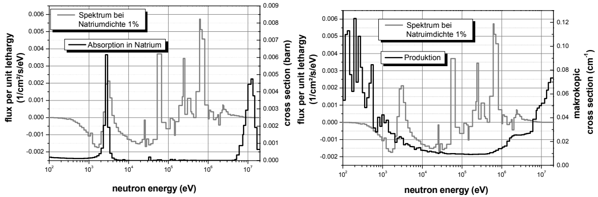
Fig. 3: Change in the neutron flux spectrum due to voiding of the sodium coolant in relation with the absorption cross section in the sodium coolant (left) and the macroscopic neutron production cross section \nu\Sigma_f - \Sigma_a (right)
