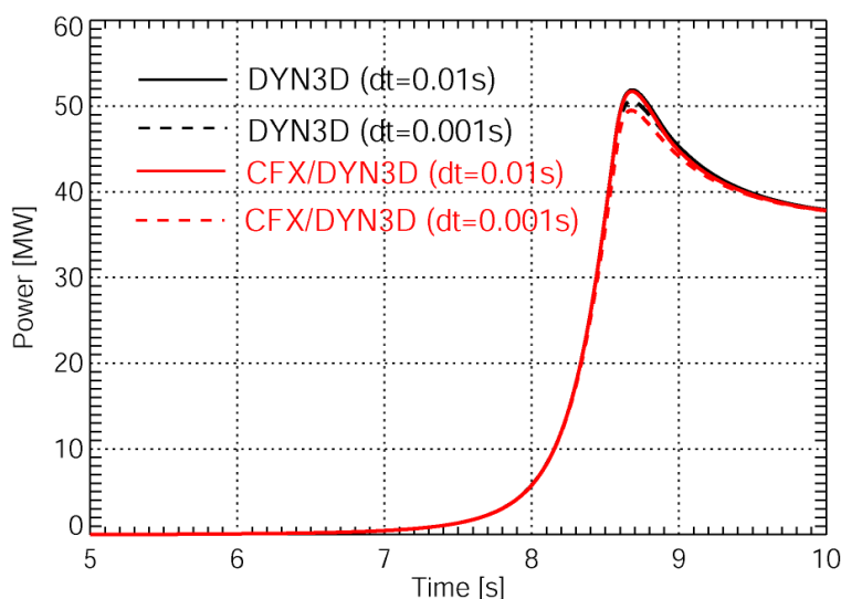
Fig. 3: Core power behavior in the DYN3D and CFX/DYN3D calculations
