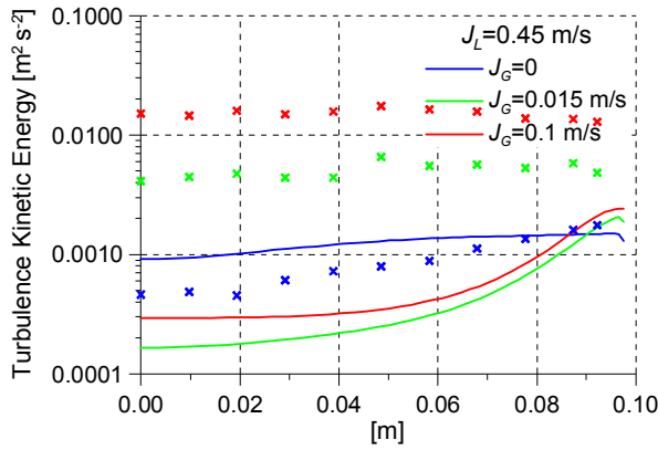
Fig. 1: Measured and calculated profiles for turbulent kinetic energy, measurements marked by asterisks
