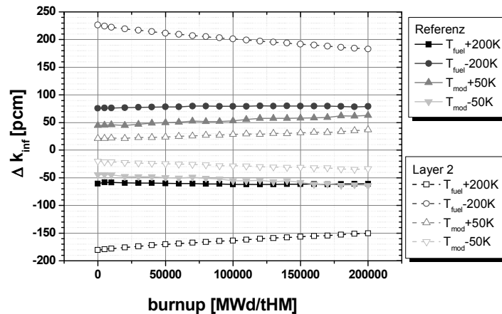
Fig. 5: Change of the fuel temperature and the coolant effect on k_{inf} over burnup for the reference case and for the system with uranium hydride layer
