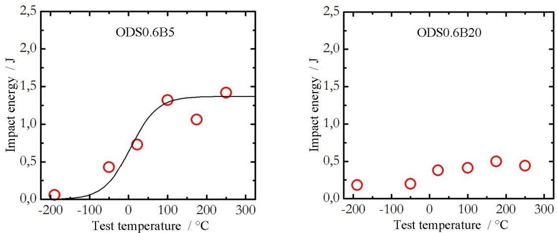
Fig. 4: Impact energy versus test temperature for ODS0.6B5 (left) and ODS0.6B20 (right)
