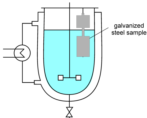
Fig. 2: Experimental set-up for batch studies
