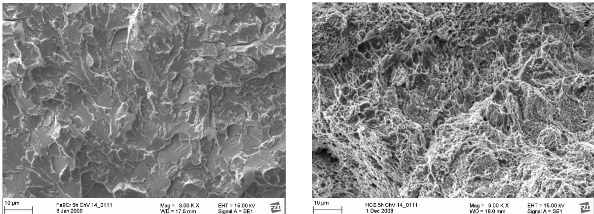
Fig. 5: Fracture appearance for FeCr5 tested at -190^{\circ}\text{C} (left) and ODS0.3A5 tested at 175^{\circ}\text{C}
