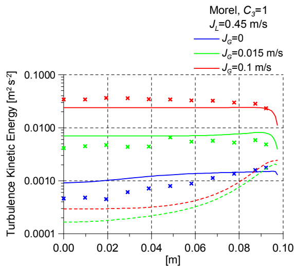
Fig. 6: CFD simulation of the profiles for turbulent kinetic energy
