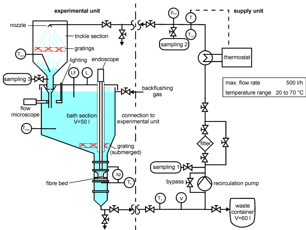
Fig. 4: Experimental set-up for long-term corrosion experiments
