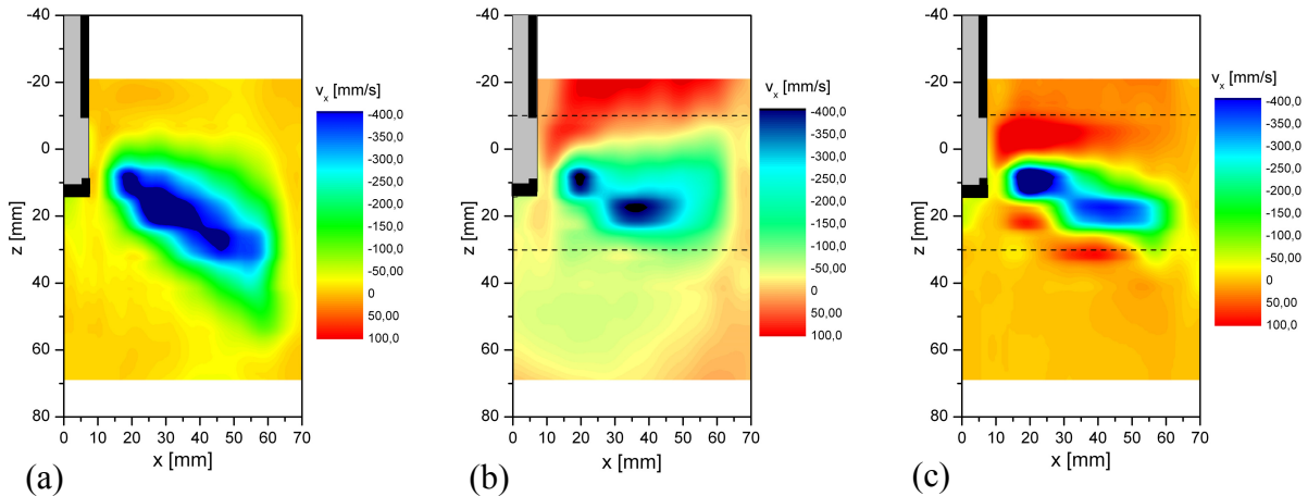
Fig. 5: Time-averaged, horizontal flow at the nozzle outlet (a) without magnetic field, (b) B = 310 \text{ mT} , non-conducting channel (c) B = 310 \text{ mT} , conducting channel
