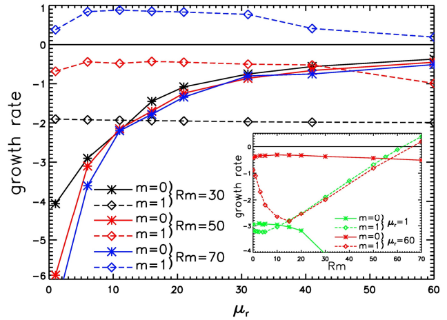
Fig. 6: Growth rates of the field amplitude (without \alpha -effect). Solid curves represent the results for the axisymmetric mode ( m=0 ) and dashed curves show the ( m=1 )-mode. The inset plot presents the growth rates for \mu_r=1 and \mu_r=60 in dependence on Rm .
