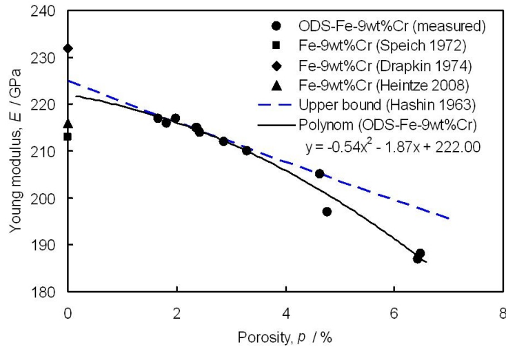
Fig. 2: Young's modulus as a function of porosity
