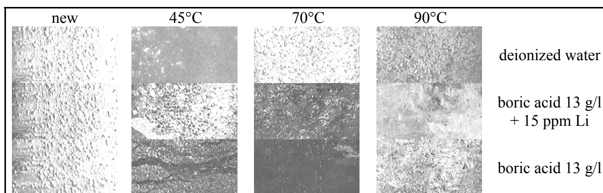
Fig. 6: Photos of sample surfaces after 7 days of treatment
