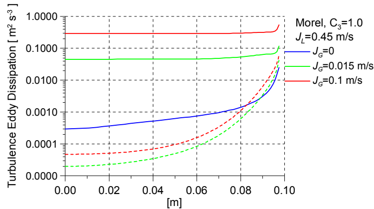
Fig. 8: CFD simulation of the profiles for turbulent eddy dissipation
