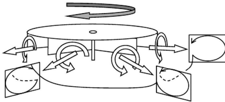
Fig. 4: Sketch of the (assumed) helical outflow in between the impeller blades providing the source for the \alpha -effect (illustration courtesy of [7])
