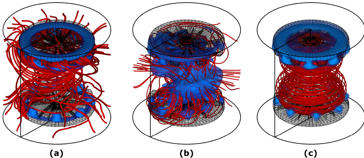
Fig. 8: Distribution of magnetic energy density (blue colored isosurfaces at 10% of the maximum value) and geometric structure of the magnetic field (red streamlines) for \mu_r=20 : (a) Rm=30 , \alpha=-1.5 , growing axisymmetric mode; (b) Rm=70 , \alpha=0 , growing ( m=1 )-mode; (c) Rm=30 , \alpha=0 , decaying axisymmetric mode. Note the ( m=8 ) modulation induced by the impeller blades.
