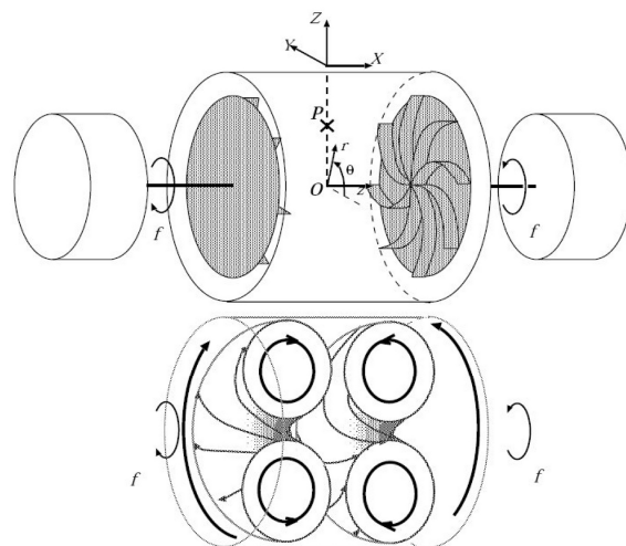
Fig. 2: Sketch of the experimental setup and the geometric structure of the basic flow
