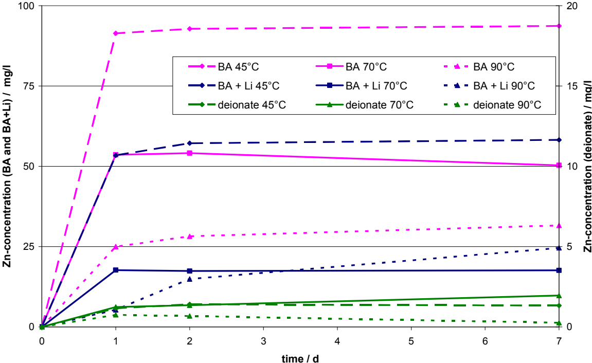
Fig. 5: Zn-concentration in solutions with deionized water (deionate), boric acid 13 g/l (BA) and boric acid 13 g/l with 15 ppm Li (BA + Li) depending on reaction time and temperature
