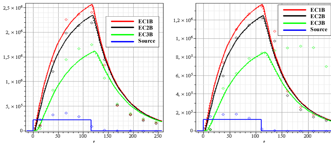
Fig. 2: Comparison of the analytical results for the space-time dependent neutron flux, using the reference element cross section set, with the experimental results for the SC3A (left) and SC3B (right) configurations of the YALINA-Booster facility
