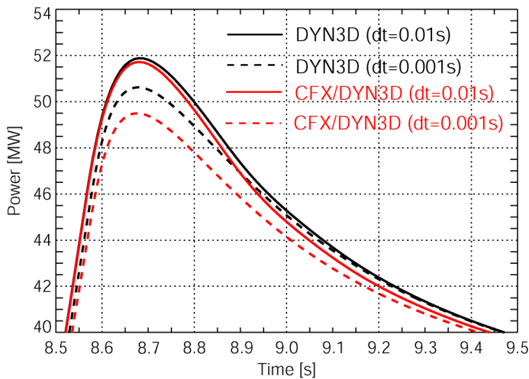
Fig. 4: Core power behavior in the DYN3D and CFX/DYN3D calculations (zoom)
