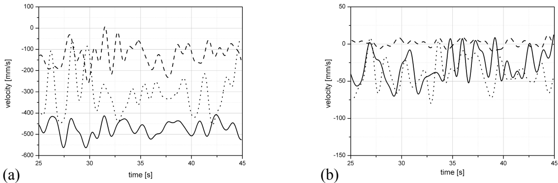
Fig. 6: Time series of the local velocity for B = 0 (solid lines), B = 310 \text{ mT} in the non-conducting mould (dotted lines) and B = 310 \text{ mT} in the conducting channel (dashed lines): (a) inside the jet; (b) below the jet
