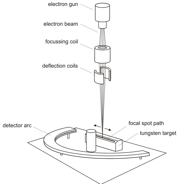
Fig. 1: Principle of ultrafast electron beam X-ray CT
