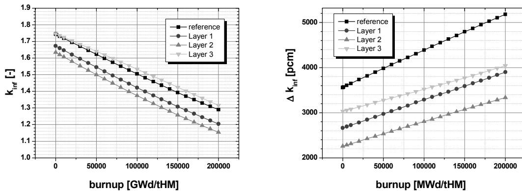
Fig. 4: Change in the infinite multiplication factor (left) and in the sodium void effect on k_{inf} over the burnup(right)
