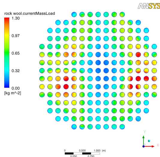
Fig. 4: Rock wool mass load [kg/m²] upper spacer grid 50s after start-up of ECC injection
