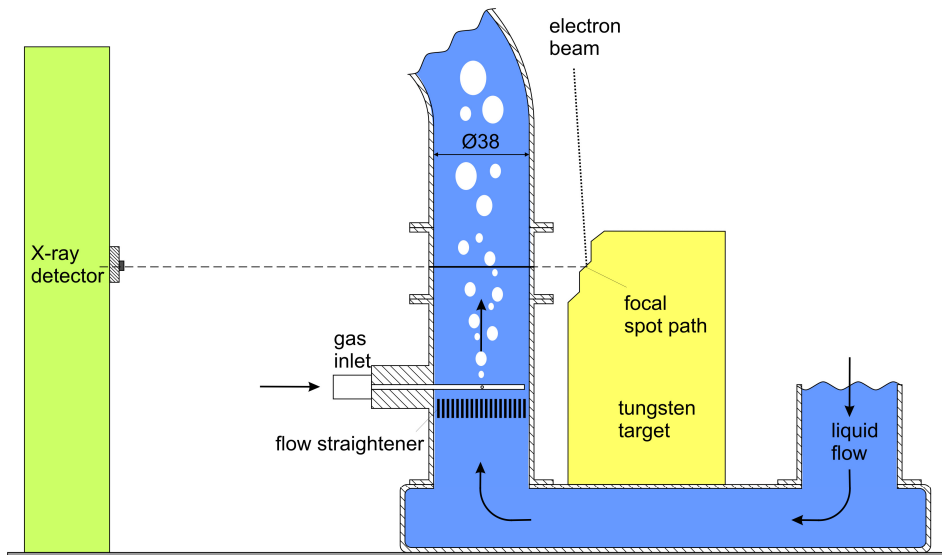
Fig. 2: Experimental two-phase flow loop setup
