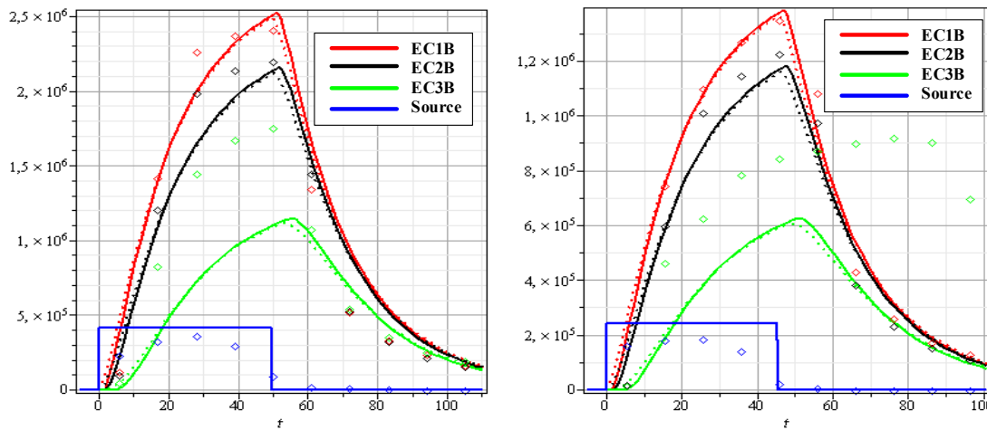
Fig. 3: Comparison of the analytical results for the space-time dependent neutron flux with the experimental results for the SC3A (left) and SC3B (right) configurations of the YALINA-Booster facility, using the fast system cross section set
