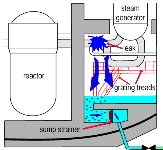
Fig. 1: Scheme of a LOCA scenario
