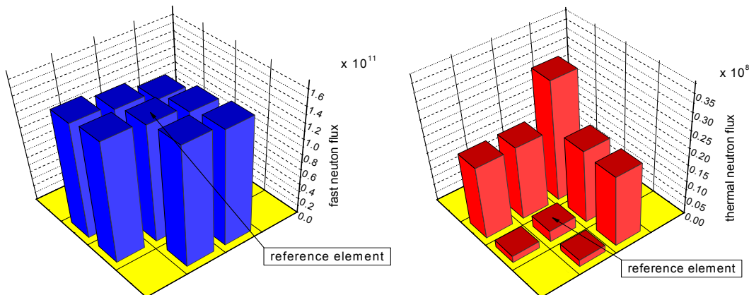
Fig. 5: Fast neutron flux (left) and thermal neutron flux (right) in the different fuel elements and areas in the fast part of YALINA-booster for SC3B
