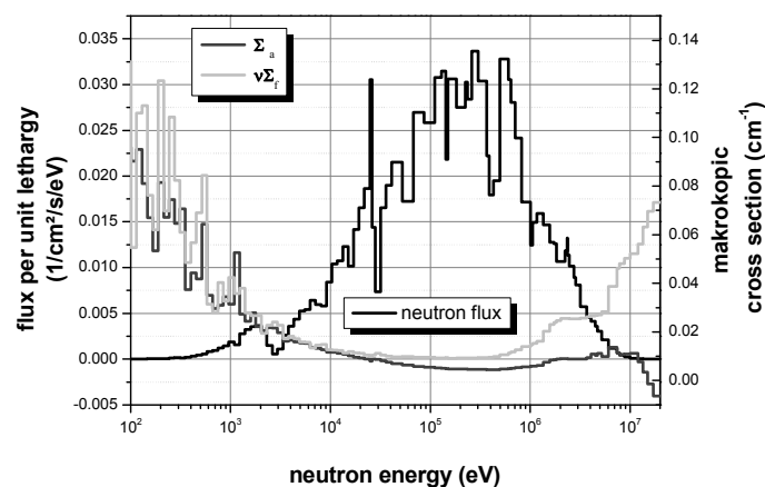
Fig. 2: Integral neutron flux spectrum and macroscopic cross sections averaged in the calculated fuel element of a sodium cooled fast reactor
