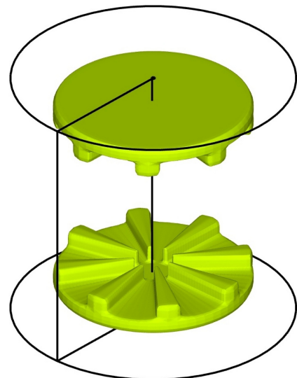
Fig. 5: Structure of the permeability distribution. The fluid permeability outside the domain indicated by the isosurface is set to \mu_r=1
