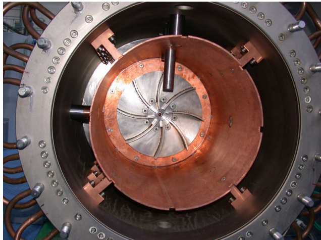
Fig. 1: Opened container of the VKS dynamo experiment. An internal copper wall is mounted within the stainless steel cylinder and separates the flow active region from the side layers
