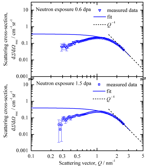
Fig. 2: Difference nuclear scattering cross sections for Fe-12.5at%Cr irradiated up to 0.6 and 1.5 dpa with the unirradiated control taken as reference
