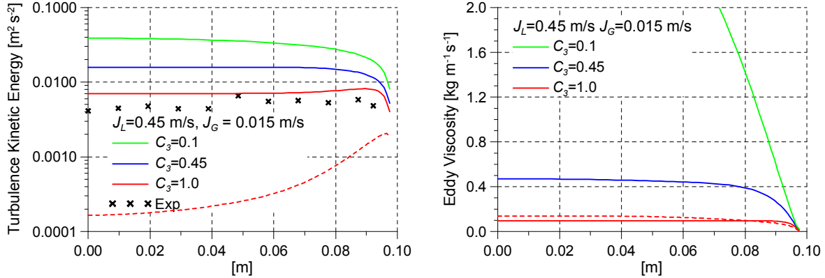
Fig. 5: Calculated profiles for turbulent kinetic energy (left) and for eddy viscosity (right) for different values of C_3 , the dotted lines mark the Sato approach (comp. Fig 1)
