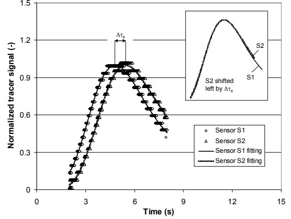
Fig. 2: Tracer signals S1 and S2 ( u_L = 0.49 \text{ cm/s} , u_G = 2.12 \text{ cm/s} , pixel position \{07;11\} )
