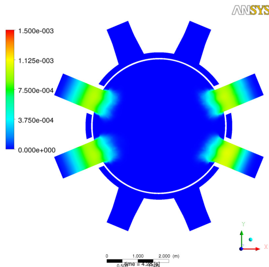
Fig. 3: Rock wool concentration [ppm] 4.3s after start-up of ECC injection, nozzle plane
