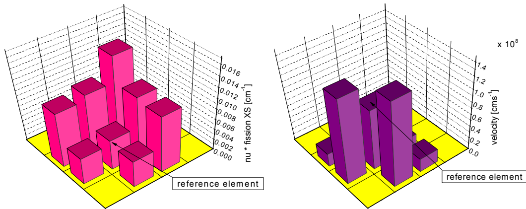
Fig. 4: Neutron production cross section (left) and neutron velocity (right) for the different fuel elements and areas in the fast part of YALINA-booster for SC3B
