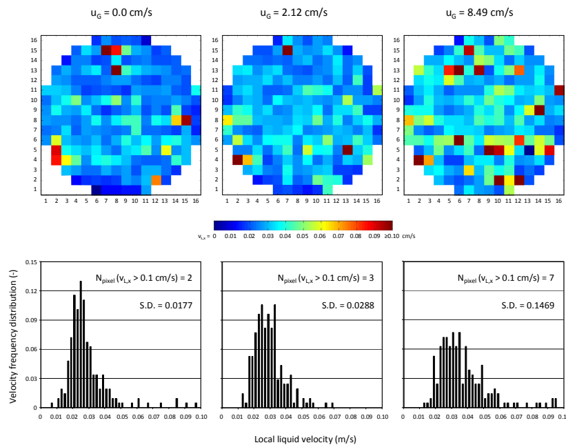
Fig. 4: Effect of superficial gas velocity on liquid velocity distribution and corresponding frequency distribution of the local liquid velocities ( u_L = 0.71 cm/s)
