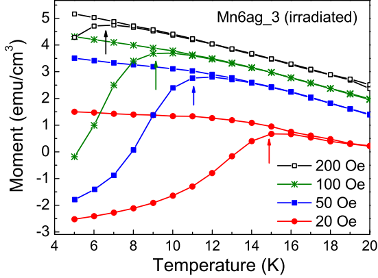
FIG. 7. ZFC/FC magnetization curves for the sample Mn6ag_3 after irradiation. The measurements were performed in different fields. The curves are vertically shifted for better visibility. The disparity between the ZFC and FC curves is the signature of superparamagnetism. The blocking temperatures (indicated by arrows) are shifted to lower temperatures with increasing measurement field.
