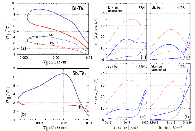
Figure 5 Calculated electrical conductivity anisotropy at 300 K of bulk (a) Bi 2 Te 3 and (b) Sb 2 Te 3 . Electron doping refers to blue lines, while red lines refer to hole doping. The dashed lines in panel (a) present the ratio obtained with an anisotropic relaxation time \tau_{\parallel}/\tau_{\perp} = 0.47 , while all other results are obtained with an isotropic relaxation time ( \tau_{\parallel} = 11 fs (12 fs) for Bi 2 Te 3 (Sb 2 Te 3 )). Experimental data (circles and triangles) are given for comparison (further details in [43]). (c)-(f) In-plane (solid lines) and cross-plane (dashed lines) doping-dependent powerfactor at 300K for (c) Bi 2 Te 3 in the Bi 2 Te 3 structure, (d) Bi 2 Te 3 in the Sb 2 Te 3 structure, (e) Sb 2 Te 3 in the Bi 2 Te 3 structure and (f) Sb 2 Te 3 in the Sb 2 Te 3 structure. Electron (hole) doping is presented as blue thick (red thin) line. The lattice constants of unstrained bulk Bi 2 Te 3 and Sb 2 Te 3 are 4.384 Å and 4.264 Å, respectively. Adapted with permission from Ref. [43], Copyright (2011) APS.
