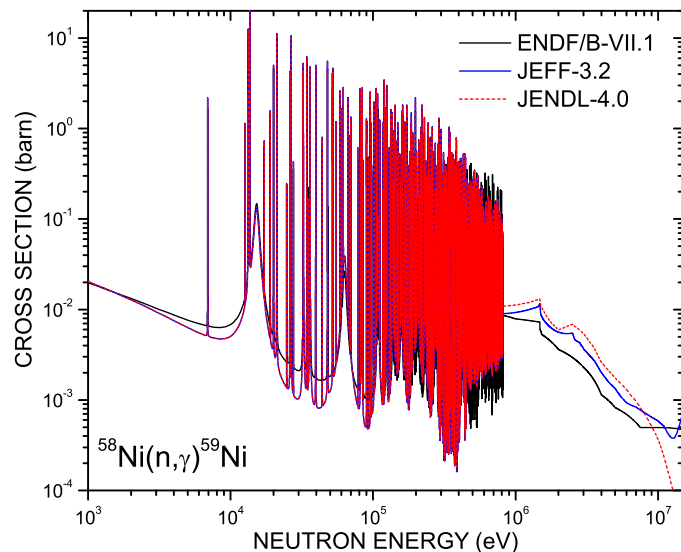
FIG. 4. (Color online) Comparison of the neutron capture cross section from the evaluated libraries ENDF/B-VII.1 [32], JEFF-3.2 [35], and JENDL-4.0 [36].
