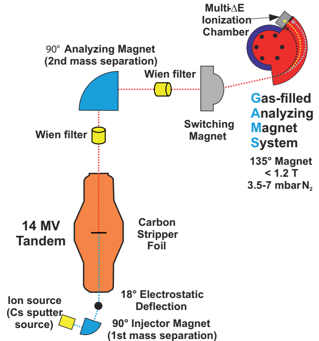
FIG. 2. (Color online) Schematic illustration of the GAMS setup at the MLL in Garching (not to scale). Blue and red dotted lines represent the negatively and positively charged ion beam of interest, respectively. In the GAMS magnet, the isotope of interest follows the yellow, dotted trajectory into the detector. Black and grey dotted lines in the GAMS magnet represent isobars of higher and lower element number Z , respectively.
