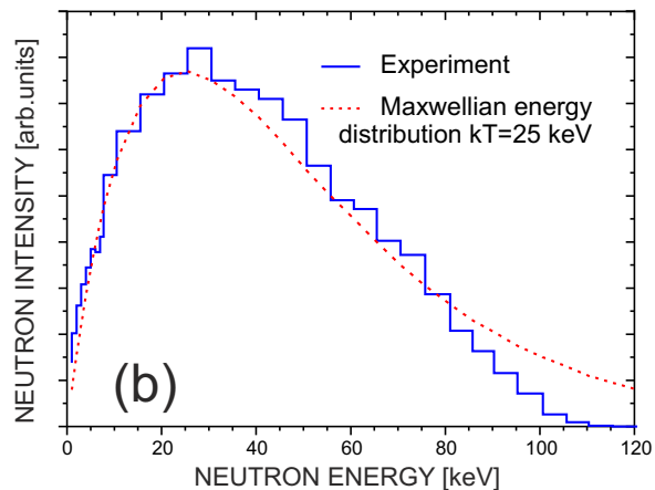
FIG. 1. (Color online) a) Schematic drawing of the neutron production target and position of the samples during irradiation. At E_p = 1912 keV the neutrons are kinematically collimated in a forward cone with 120^\circ opening angle. b) Comparison of the experimental neutron spectrum with a Maxwellian energy distribution of kT = 25 keV.
